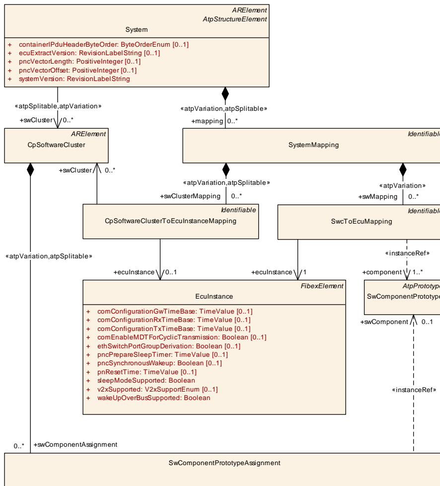
Figure 5.32: Visualization of constr_5219
