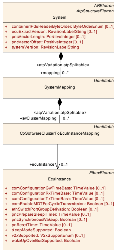
Figure 5.30: Modeling of the CpSoftwareClusterToEcuInstanceMapping
