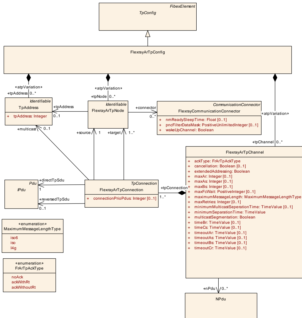
Figure 6.60: FlexRay Autosar Transport Layer Configuration (TransportProtocols: FlexRayAutosarTransportProtocol)
