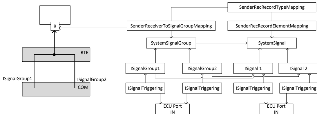
Figure 6.92: Scenario where RTE does perform a fan-in for a SystemSignalGroup
