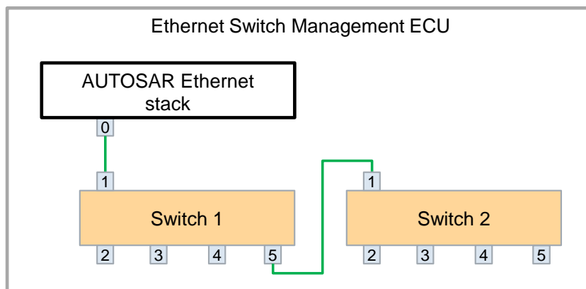
Figure 5.27: Example of managed Ethernet switches
