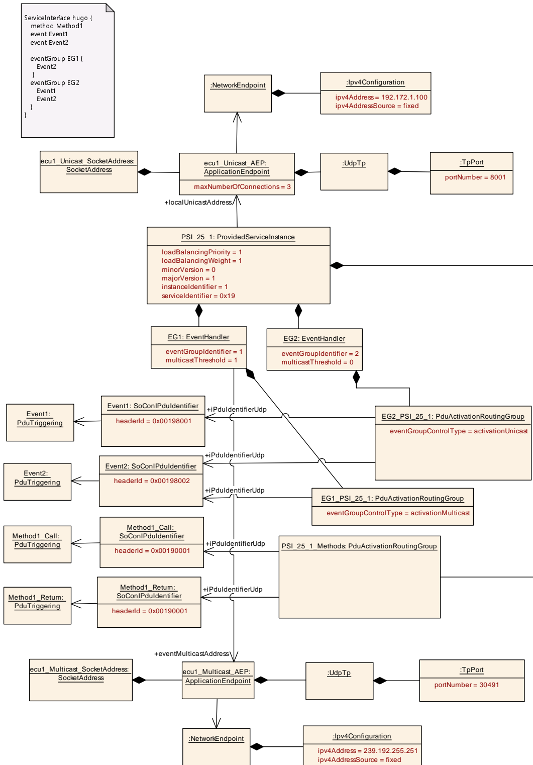
Figure 6.42: Example for the modeling of a ProvidedServiceInstance that is deployed on a local Unicast Endpoint
