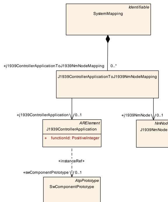
Figure 5.6: J1939 Controller Application to J1939NmNode Mapping
