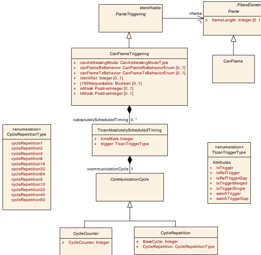
Figure 6.35: TtcanAbsolutelyScheduledTiming (Fibex4Ttcan:TtcanCommunication)
