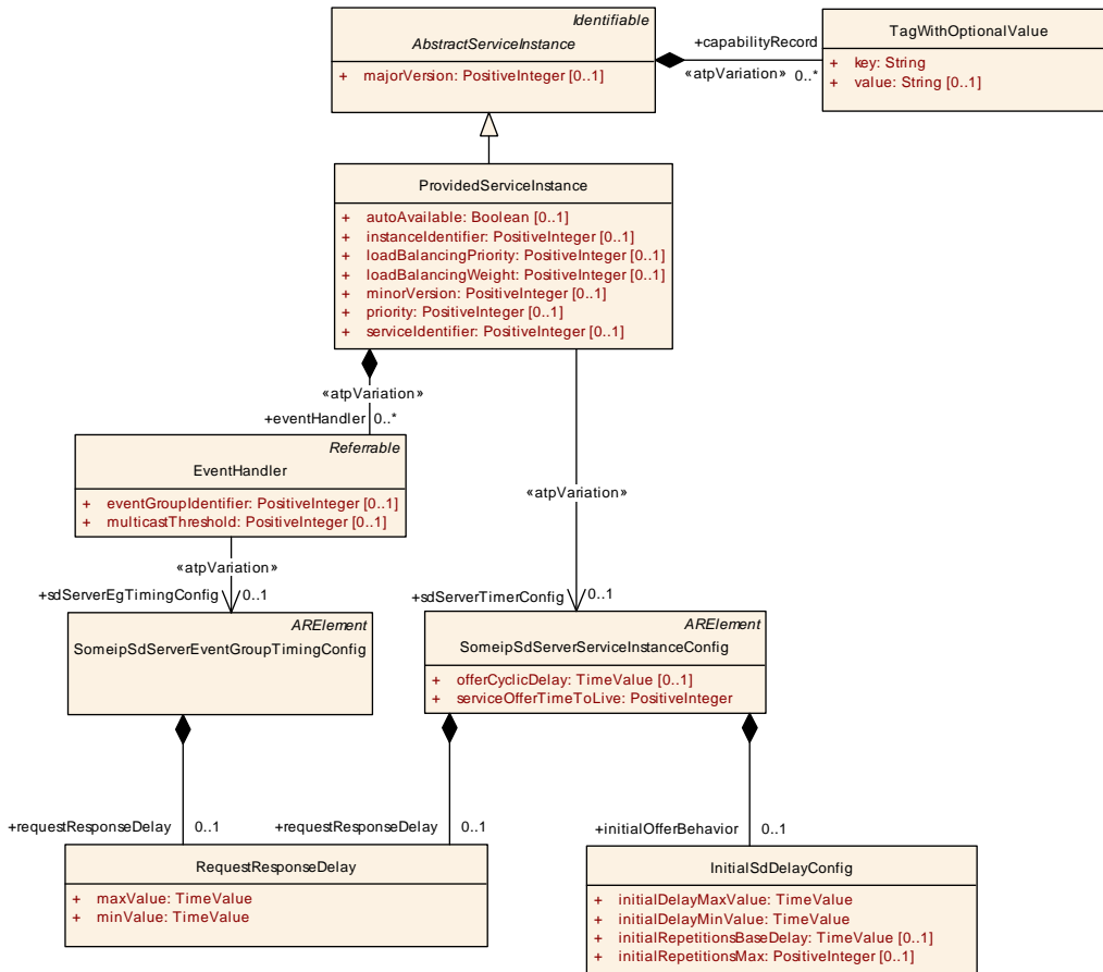
Figure 6.45: Model of SD Server Timing
