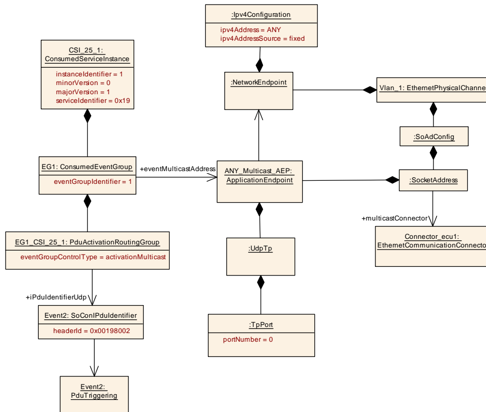
Figure 6.44: Example for the modeling of a ConsumedServiceInstance that is receiving Events over multicast only
