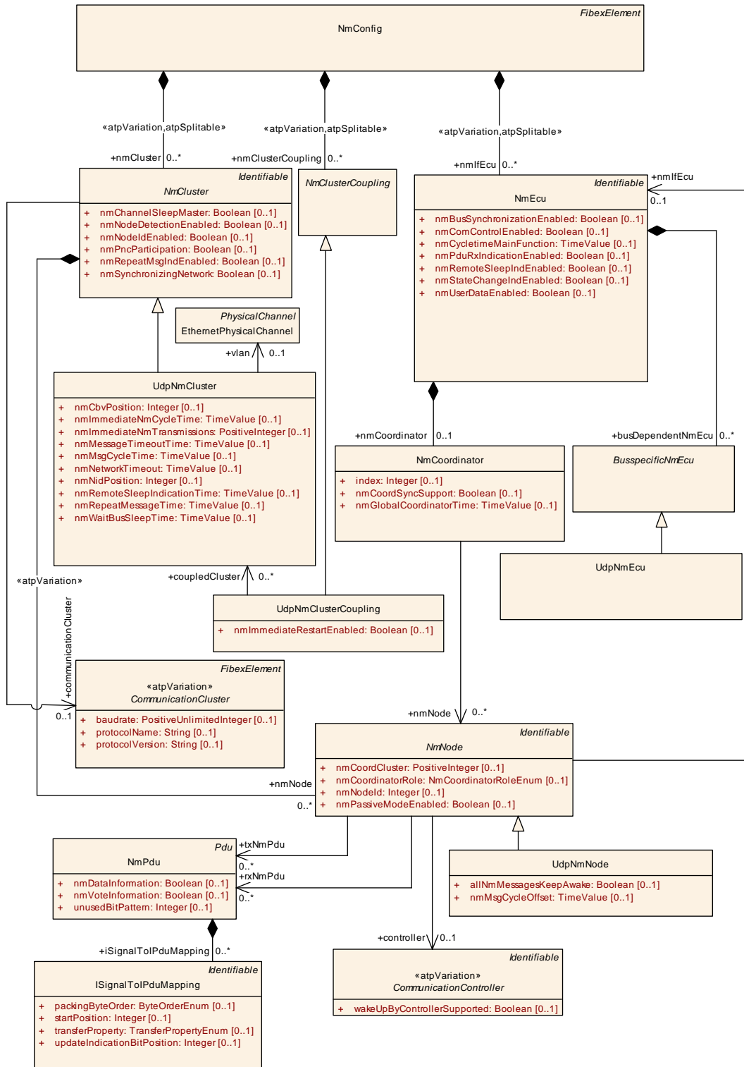
Figure 6.74: UDP Network Management Configuration (TransportProtocols: NmUdpCon-figuration)
