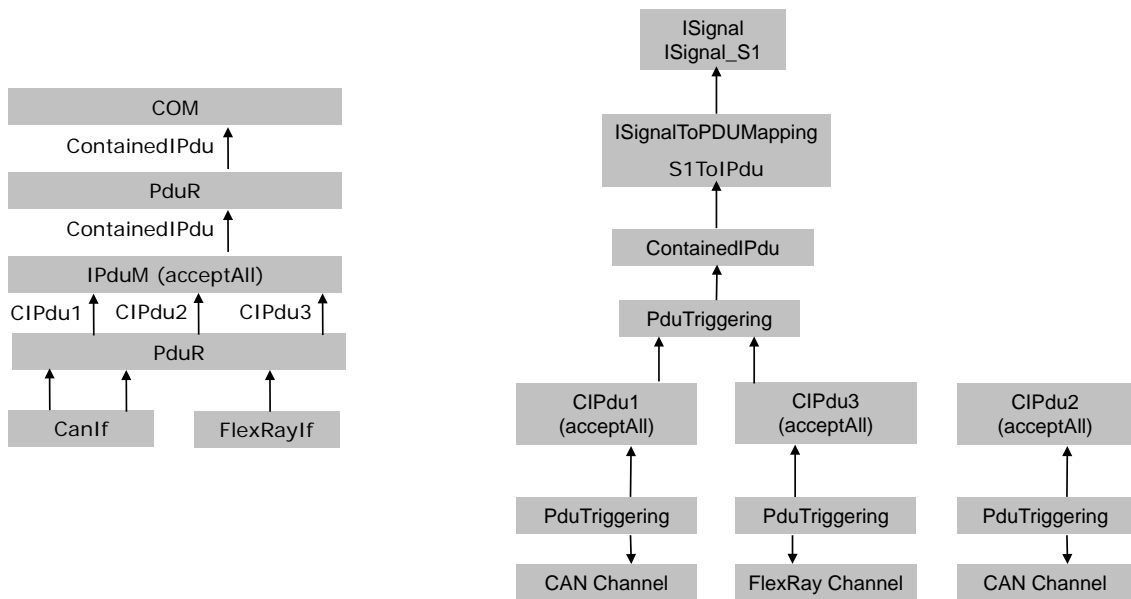
Figure 6.93: Container acceptAll fan-in
