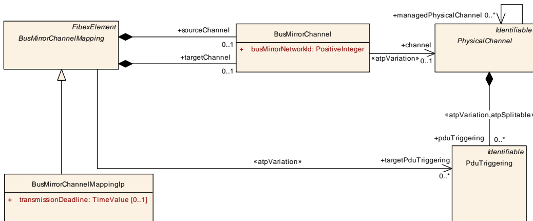
Figure 6.80: Bus mirroring between a CAN, LIN or FlexRay sourceChannel and an Ethernet IP targetChannel
