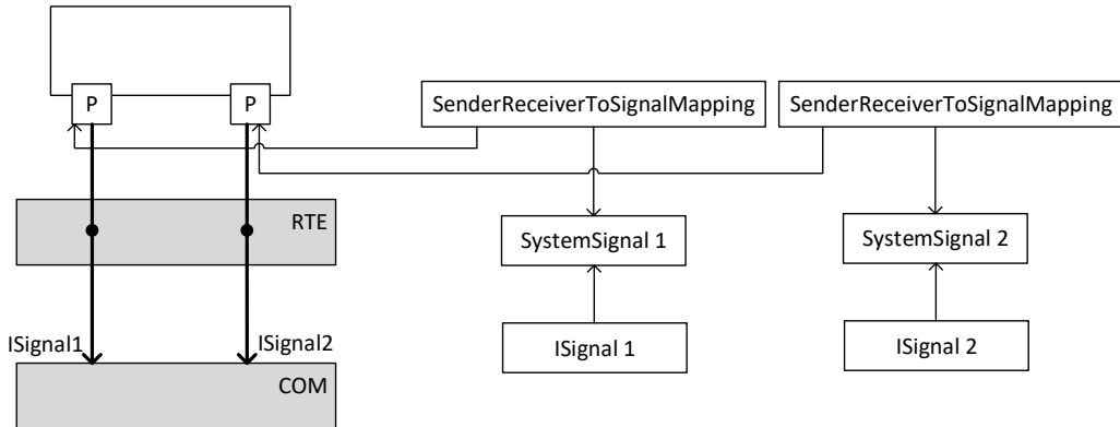
Figure 6.82: Scenario where RTE does not perform a fan-out
