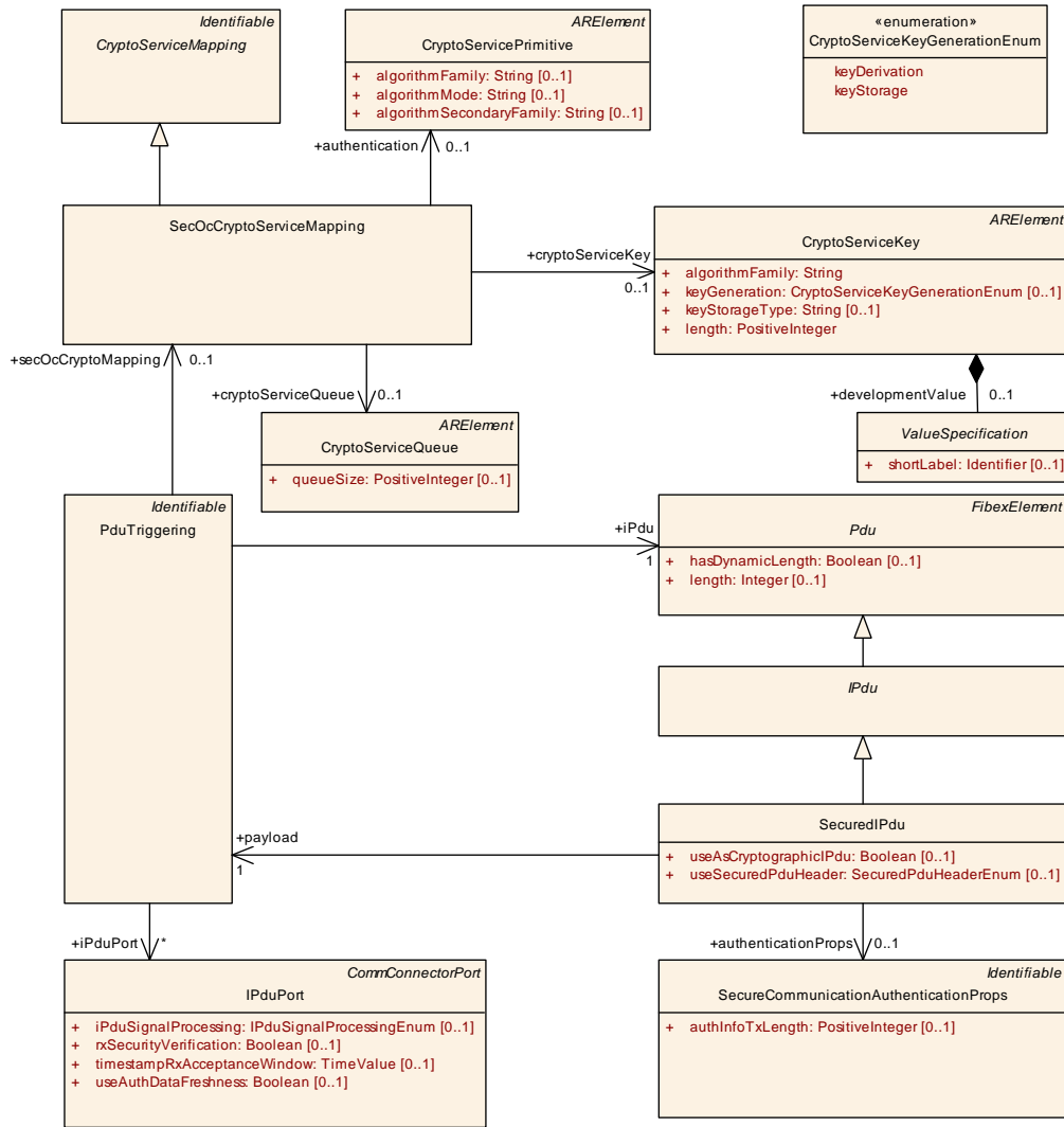
Figure 6.17: Modeling of crypto infrastructure for SecuredIPdu
