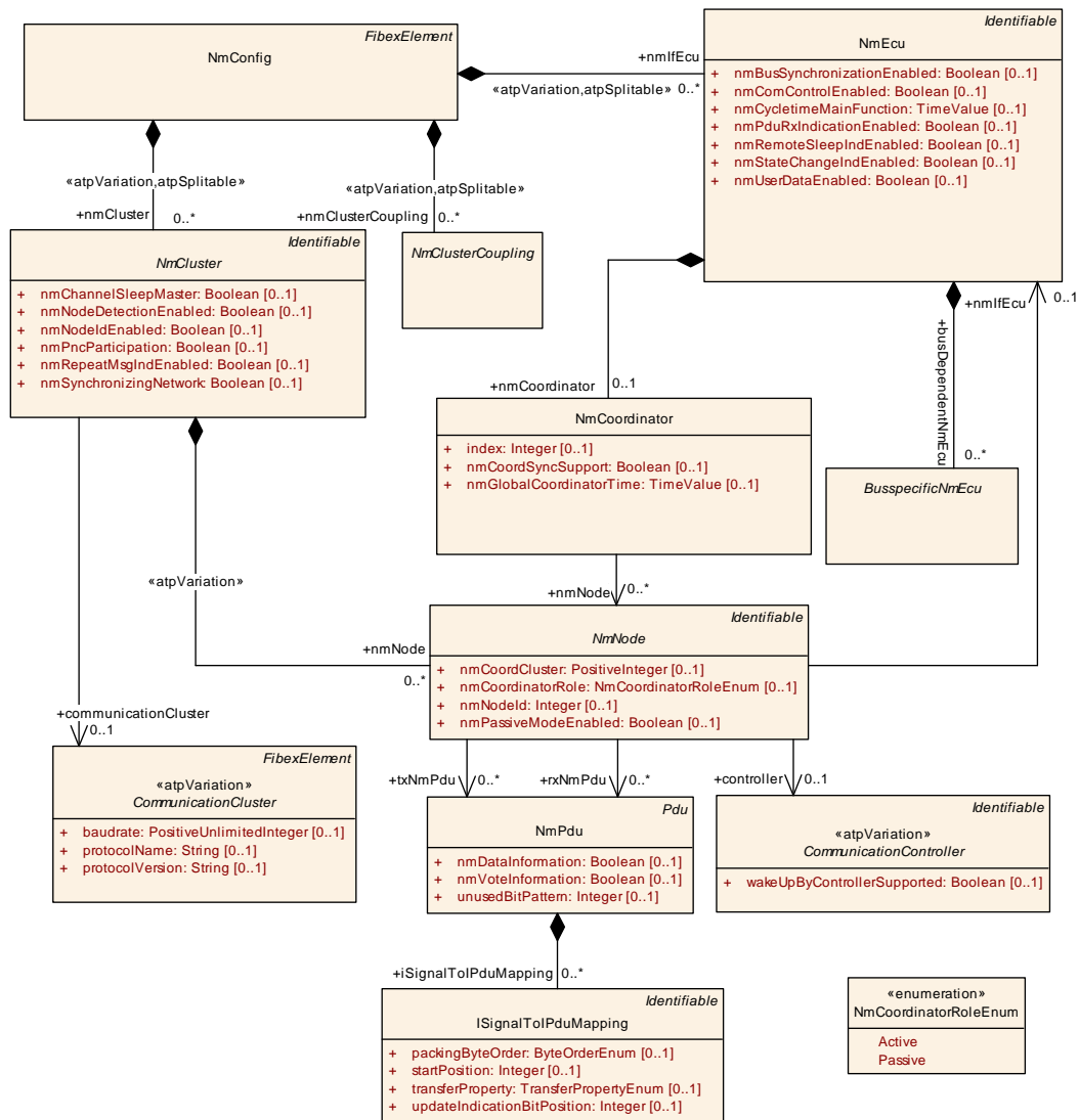
Figure 6.69: Generic Nm elements
