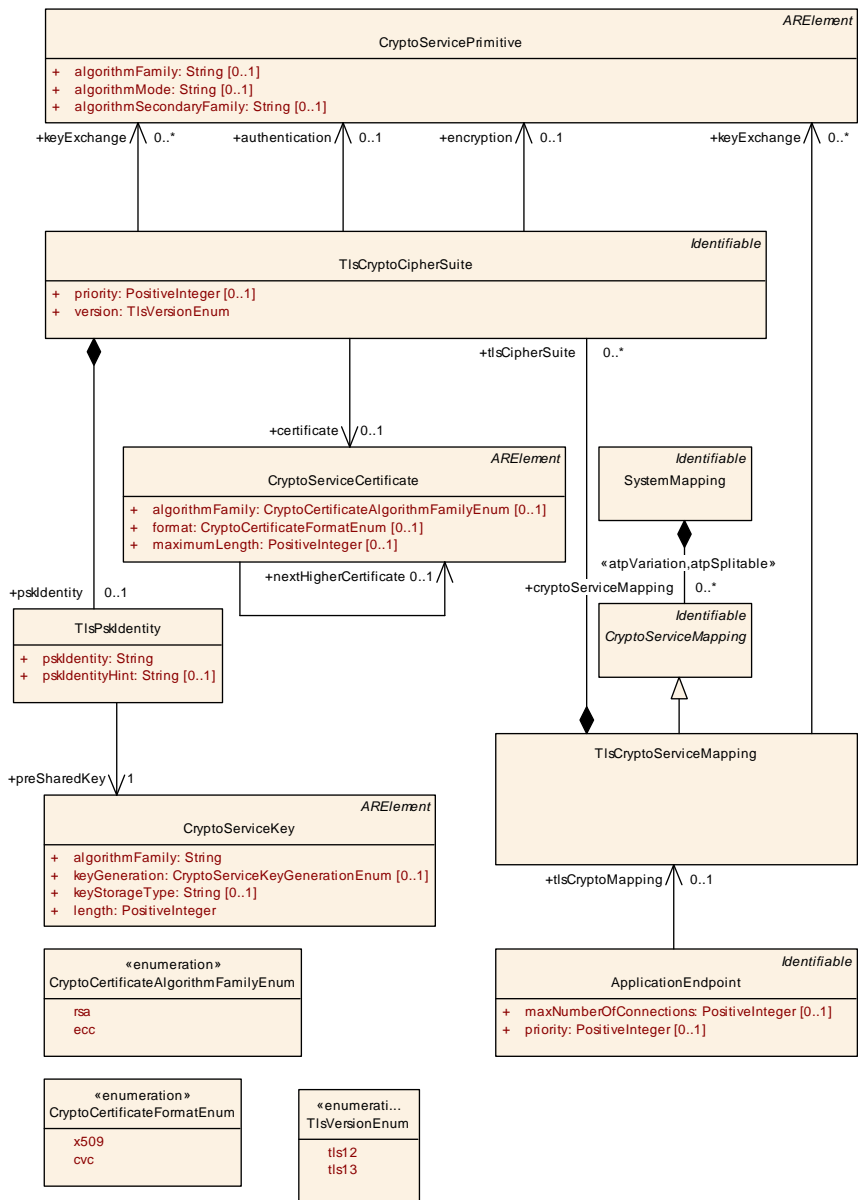
Figure 6.54: Modeling of crypto infrastructure for Transport Layer Security
