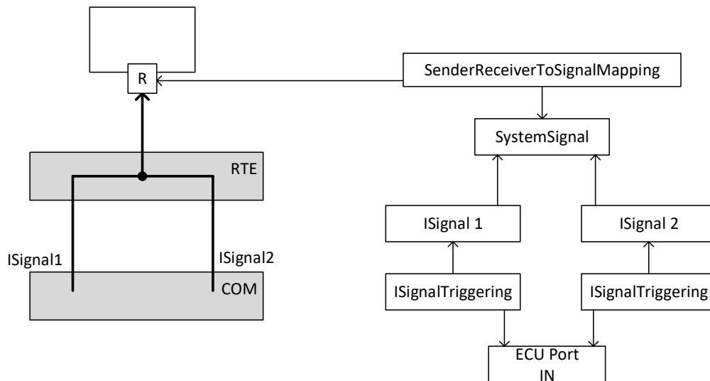
Figure 6.91: Scenario where RTE does perform a fan-in
