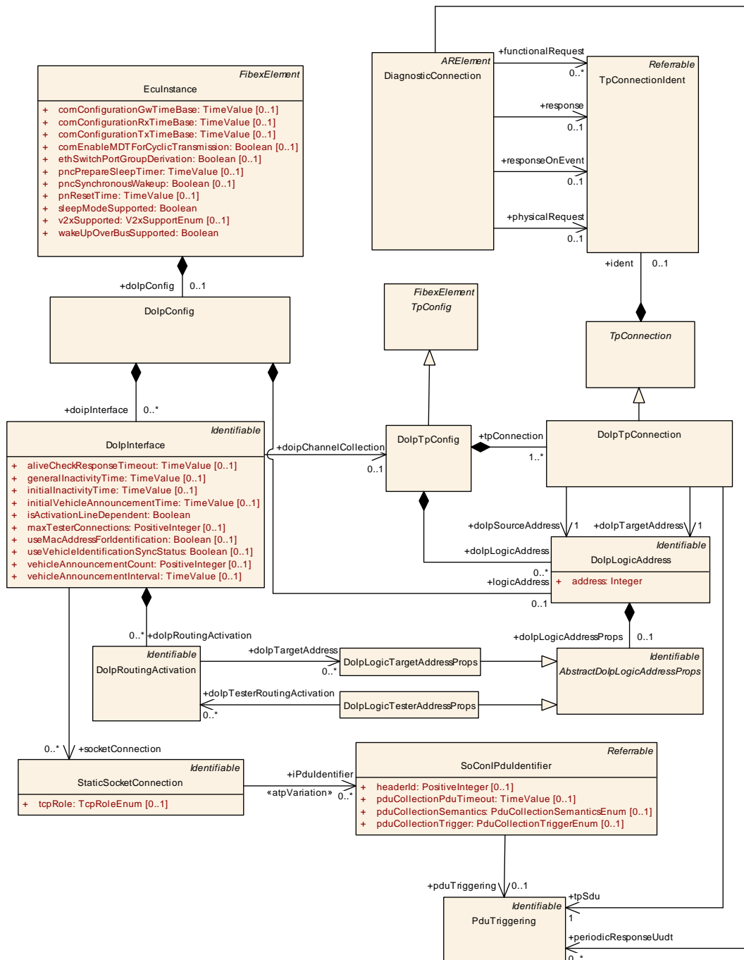
Figure 6.52: DoIP
