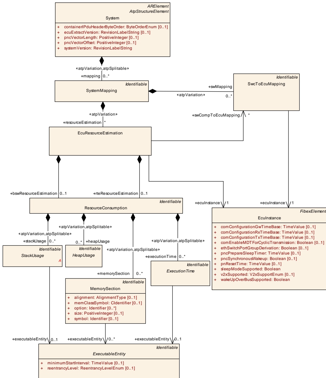
Figure 5.23: ECU resource estimations (ResourceEstimation)
