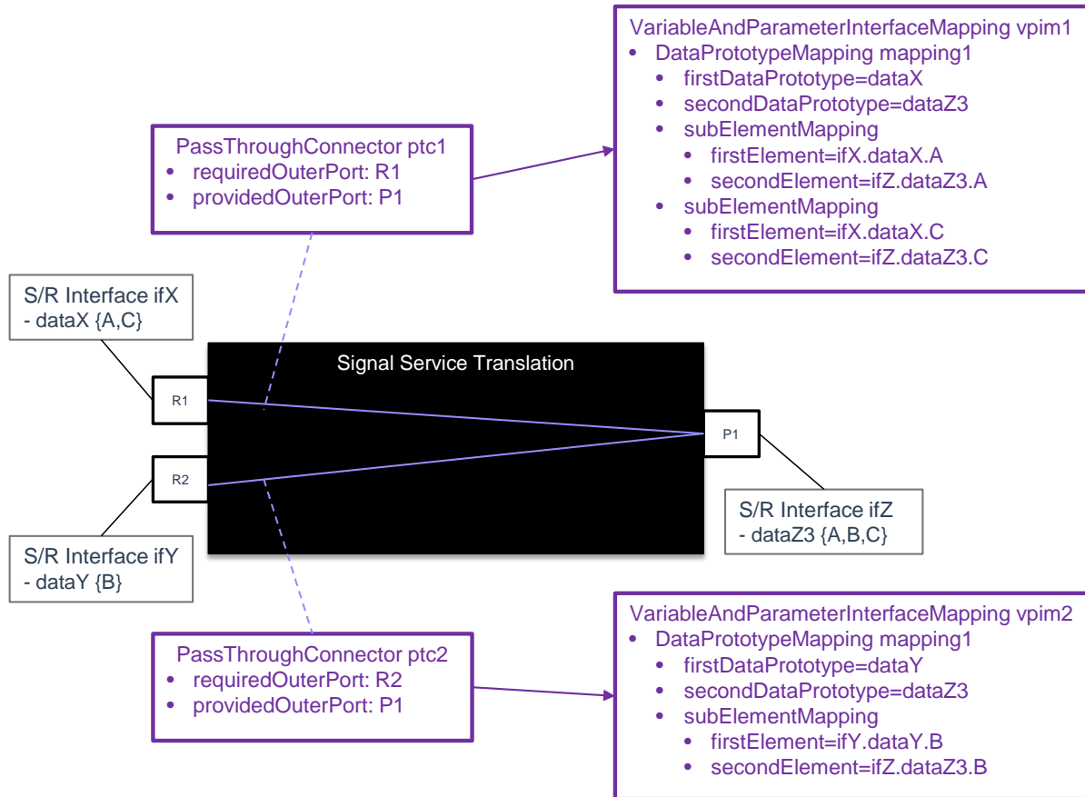
Figure 6.102: Mapping description using PassThroughSwConnectors and PortInterfaceMappings from several sources
