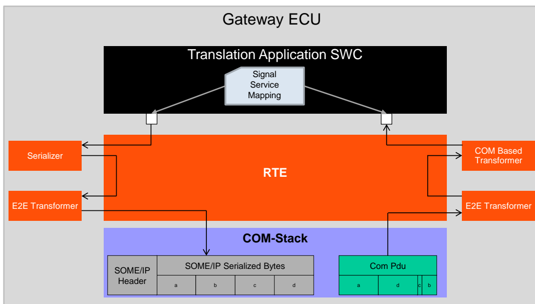
Figure 6.98: Signal Service Translation Application Software Component
