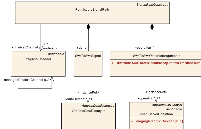
Figure 5.21: Description of the signal path that a signal shall take in the topology (PermissibleSignalPath)
