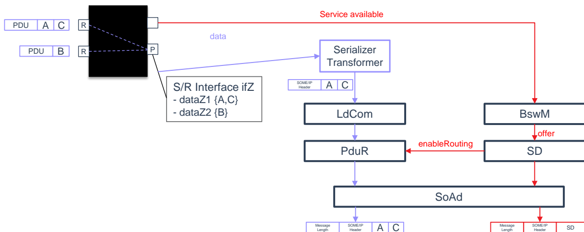
Figure 6.104: Interaction between translation SWC and Service Discovery
