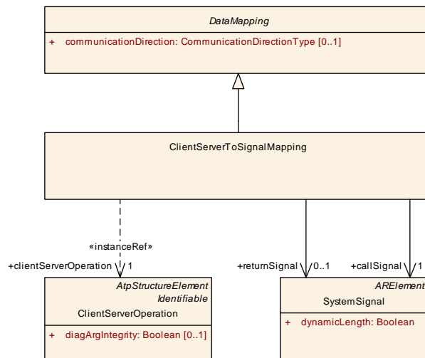
Figure 5.14: Mapping of a ClientServerOperation to a callSignal and a returnSignal
