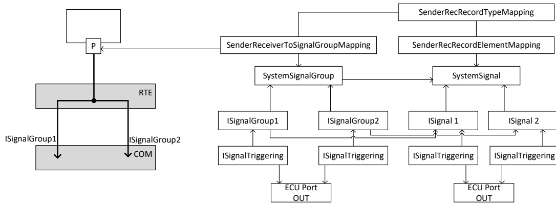
Figure 6.85: Scenario where RTE does perform a fan-out for a SystemSignalGroup
