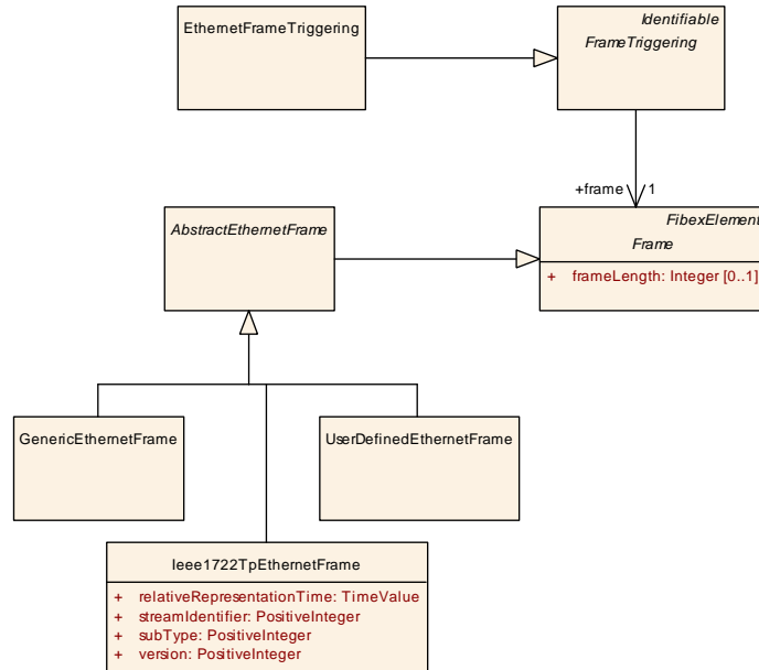
Figure 6.56: EthernetFrameType based communication
