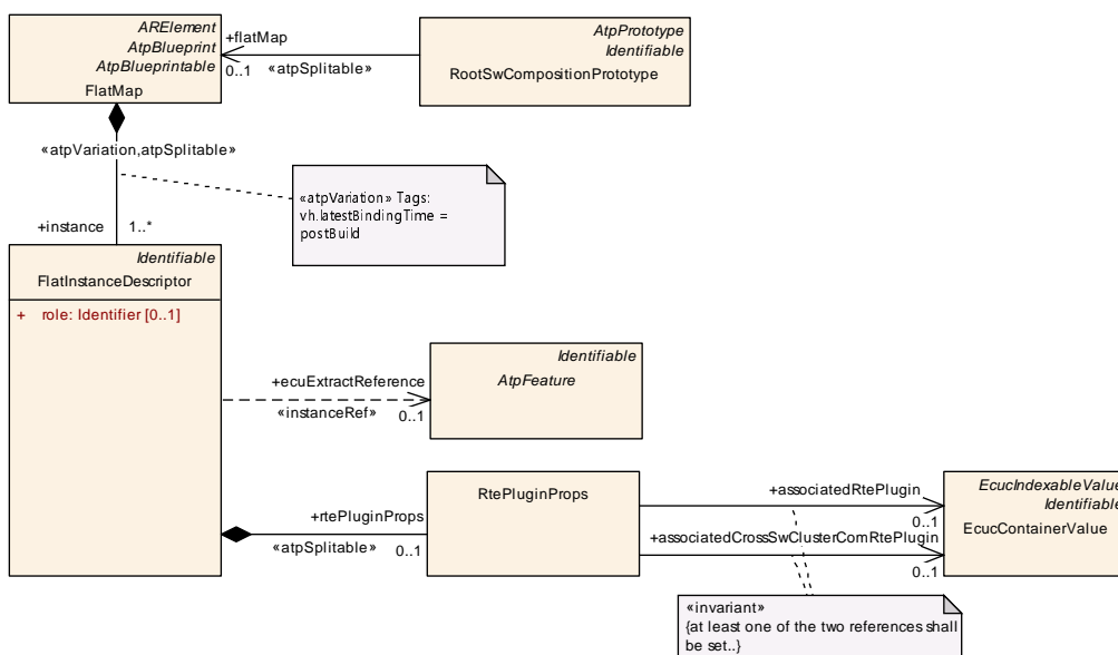
Figure 14.9: ECU Flat Map and rtePluginProps
