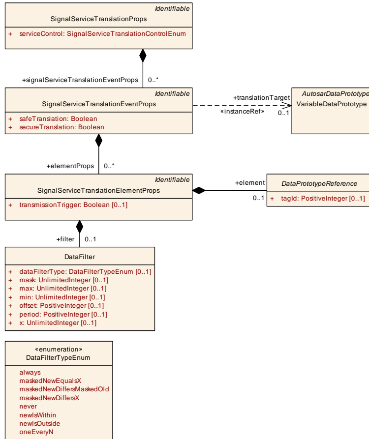
Figure 6.103: Signal Service Translation element properties
