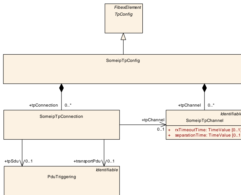
Figure 6.64: SOME/IP Segmenter
