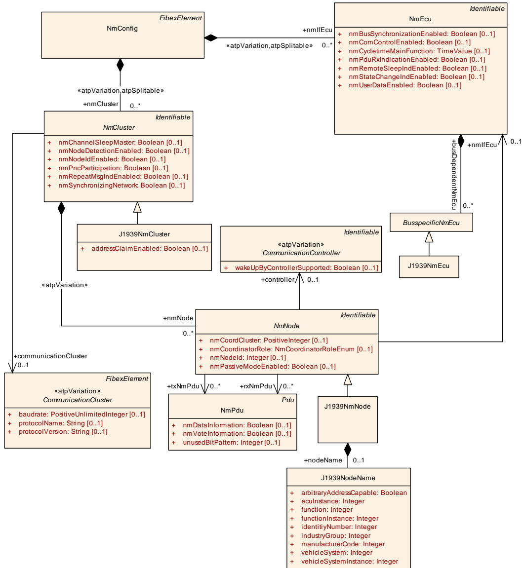
Figure 6.75: J1939 Network Management Configuration (TransportProtocols: NmJ1939Configuration)
