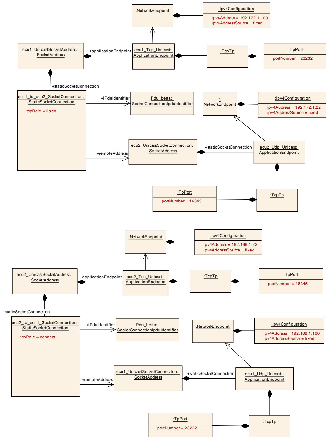
Figure 6.49: Example for the modeling of TCP StaticSocketConnections in TCP server role and TCP client role
