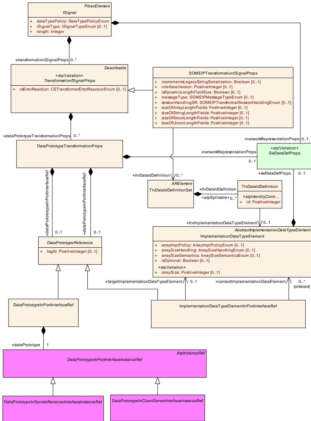
Figure 7.13: Transformer Network Representation
