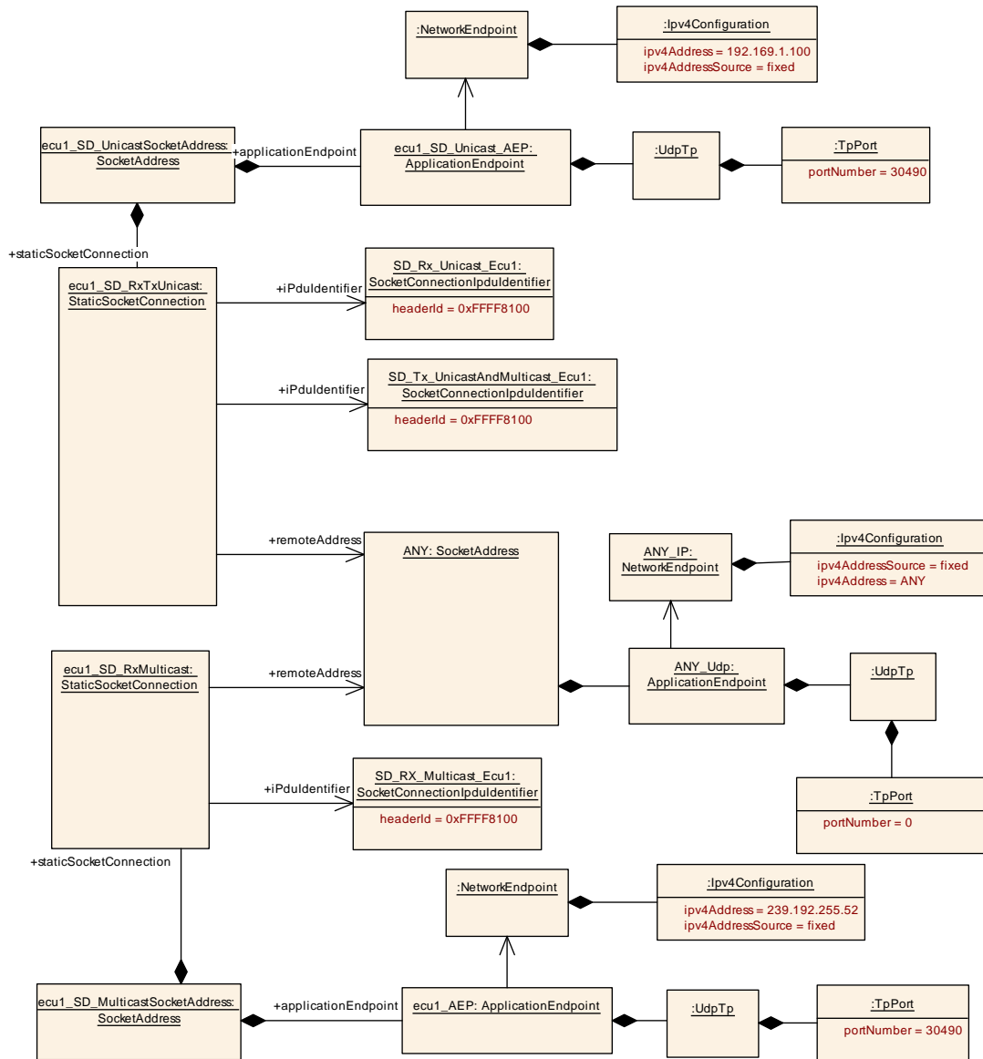
Figure 6.50: Example for the modeling of SD StaticSocketConnections
