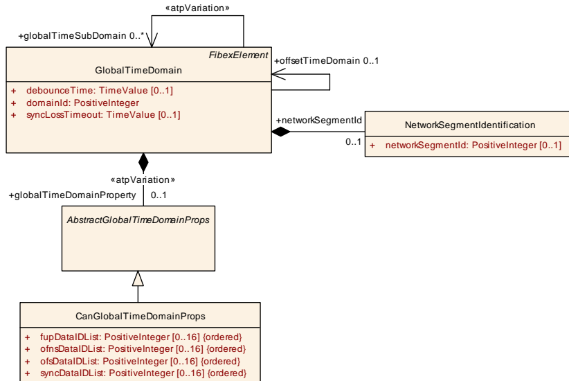
Figure 9.17: Modeling of the FlexRay specific FrGlobalTimeDomainProps
