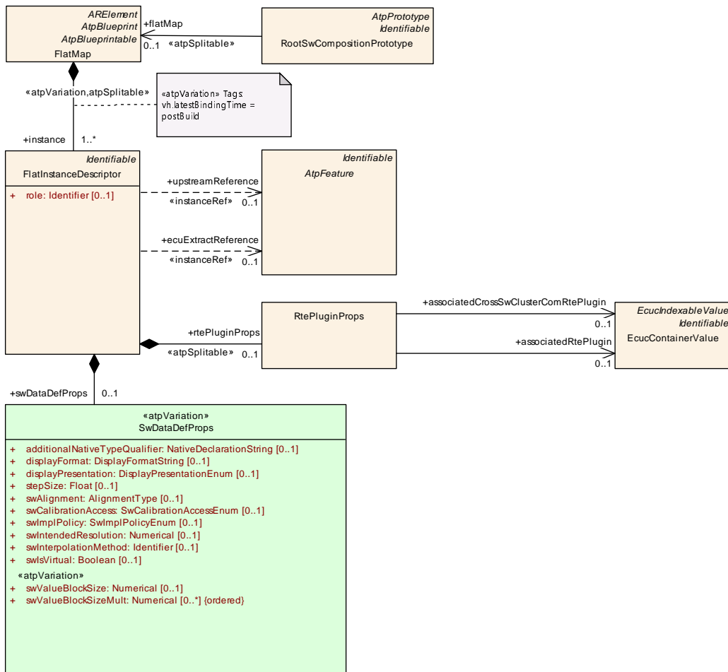
Figure 14.7: Flat Map (CommonStructure: FlatMap)
