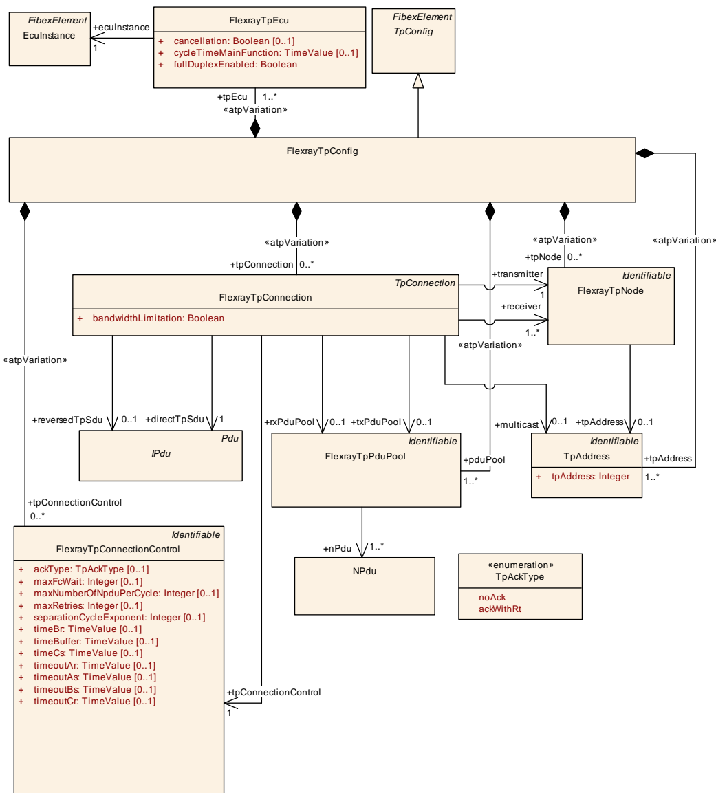
Figure 6.58: FlexRay ISO Transport Layer Configuration (TransportProtocols: FlexRay-IsoTransportProtocol)
