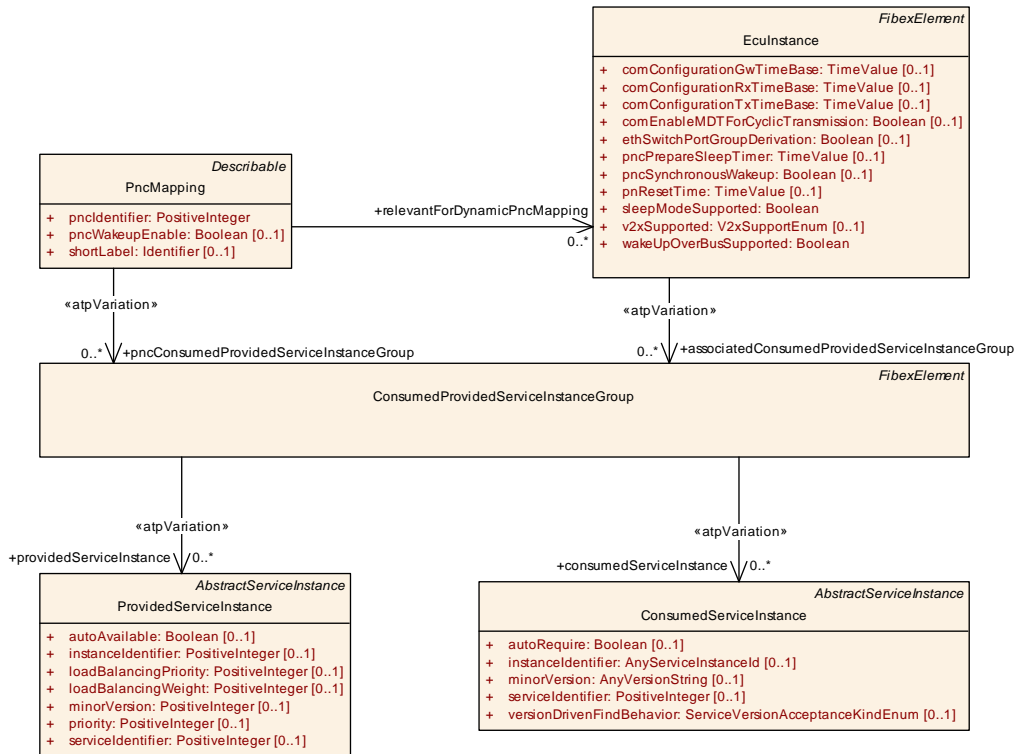
Figure 6.47: ConsumedProvidedServiceInstanceGroup
