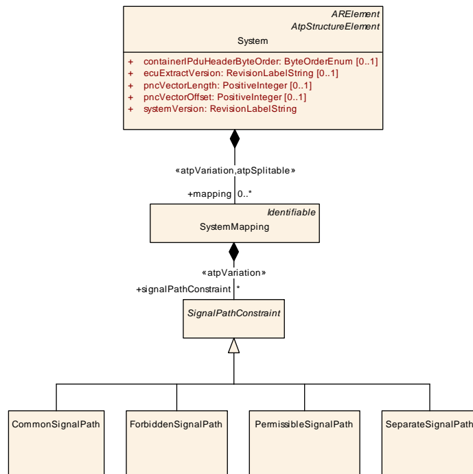
Figure 5.18: Communication Path Description (SignalPathConstraints)
