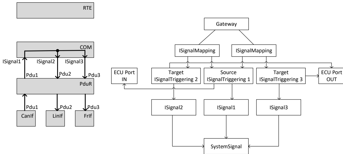
Figure 6.86: Scenario where the Com Gateway performs a fan-out and RTE is not involved
