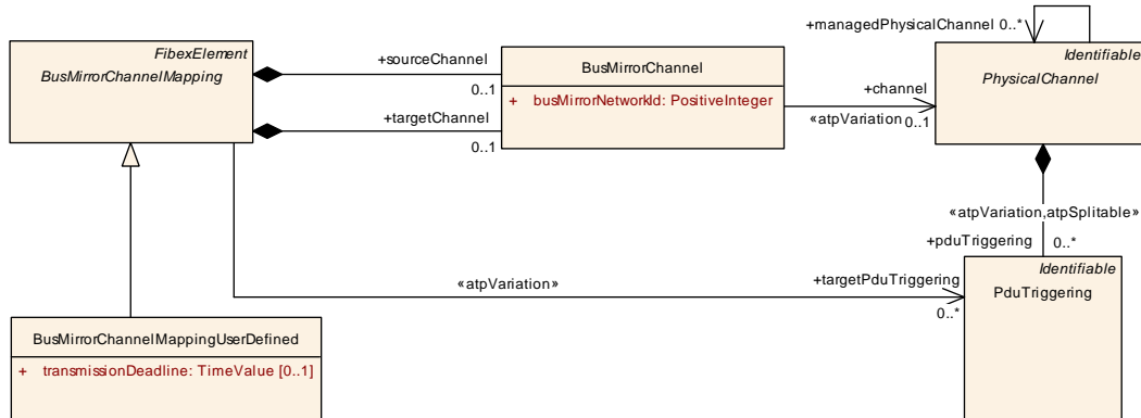
Figure 6.81: Bus mirroring between a CAN, LIN or FlexRay sourceChannel and a UserDefined targetChannel
