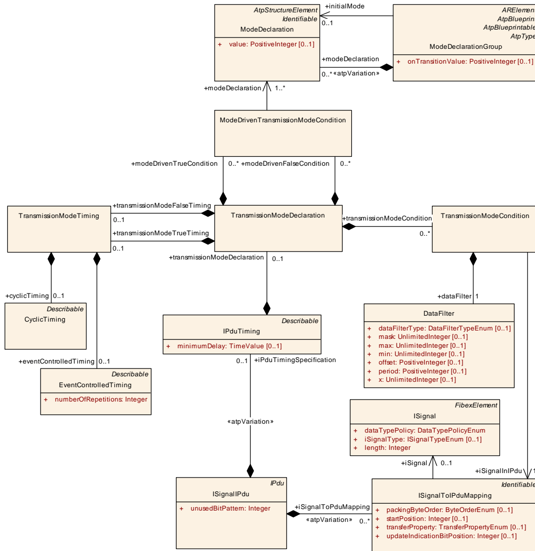
Figure 6.20: IPdu Timing
