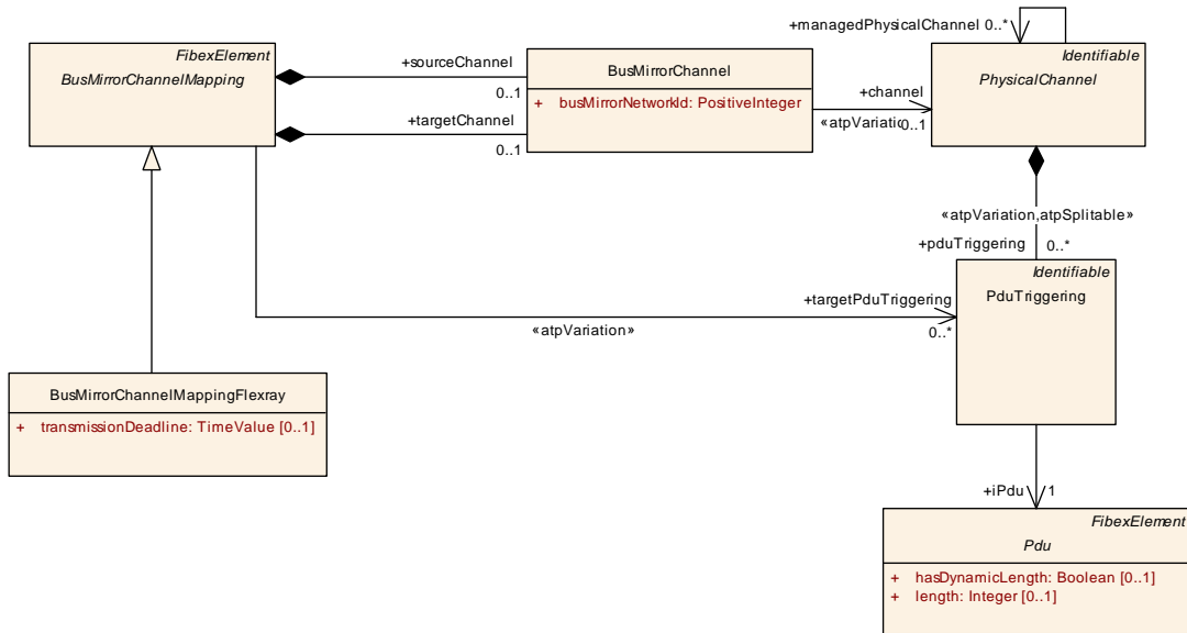
Figure 6.79: Bus mirroring between a CAN, LIN or FlexRay sourceChannel and a FlexRay targetChannel
