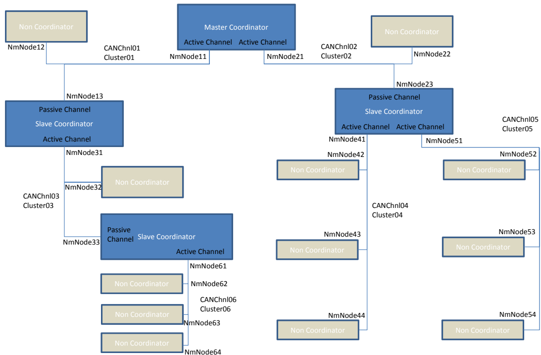
Figure 6.70: Nm Example
