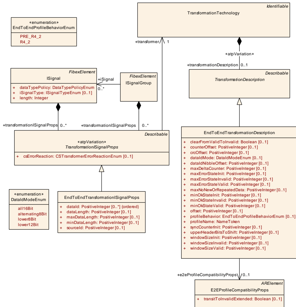
Figure 7.20: E2E Transformer Configuration
