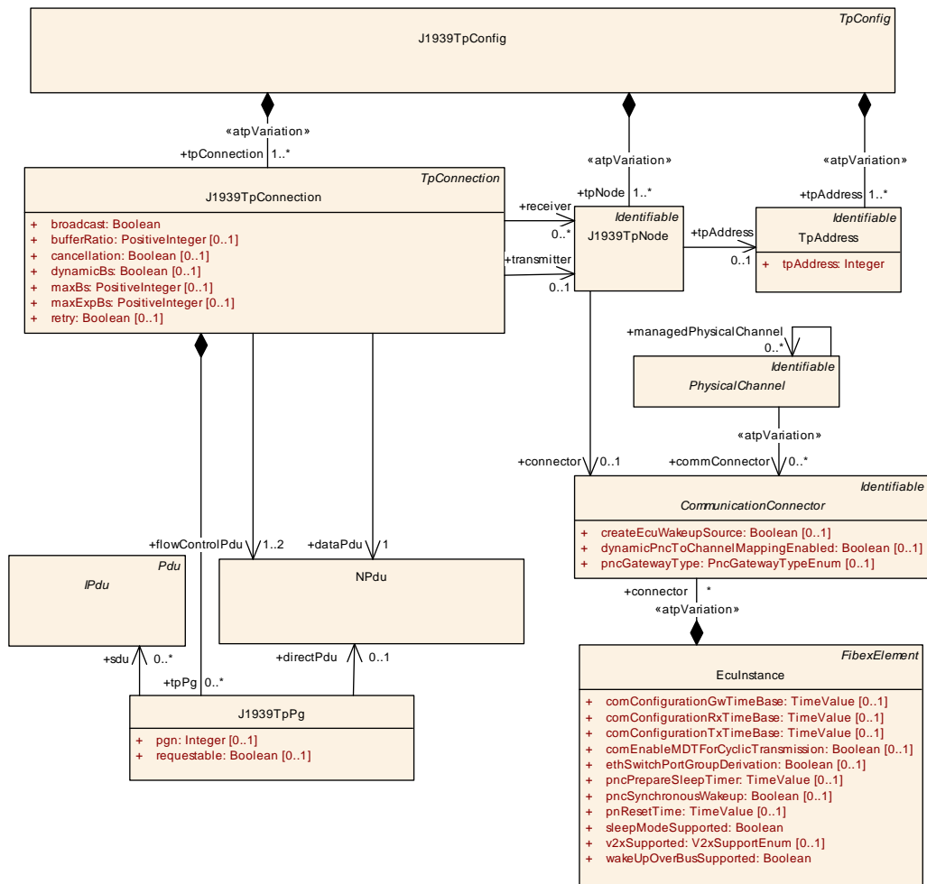
Figure 6.65: J1939 Transport Layer Configuration
