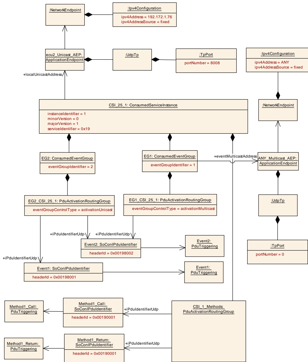
Figure 6.43: Example for the modeling of a ConsumedServiceInstance that is deployed on a local Unicast Endpoint
