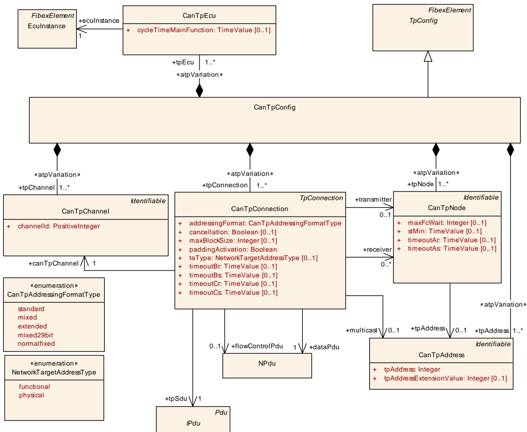
Figure 6.61: CAN Transport Layer Configuration (TransportProtocols: CanTransportProtocol)
