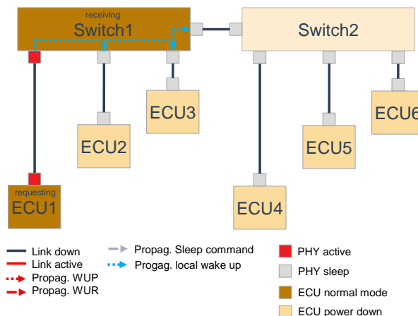
Figure 3.21: Switch1 is woken up by the PHY that received the wake-up. The received wake-up on the network is forwarded as local wake-up to the neighboring PHYs
