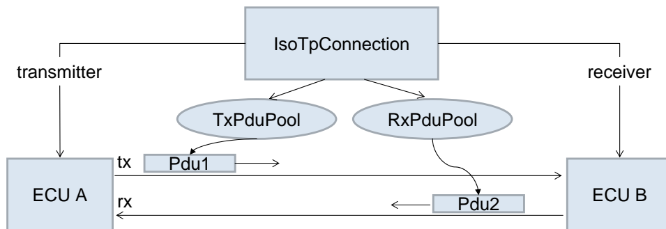
Figure 6.59: IsoTp Example
