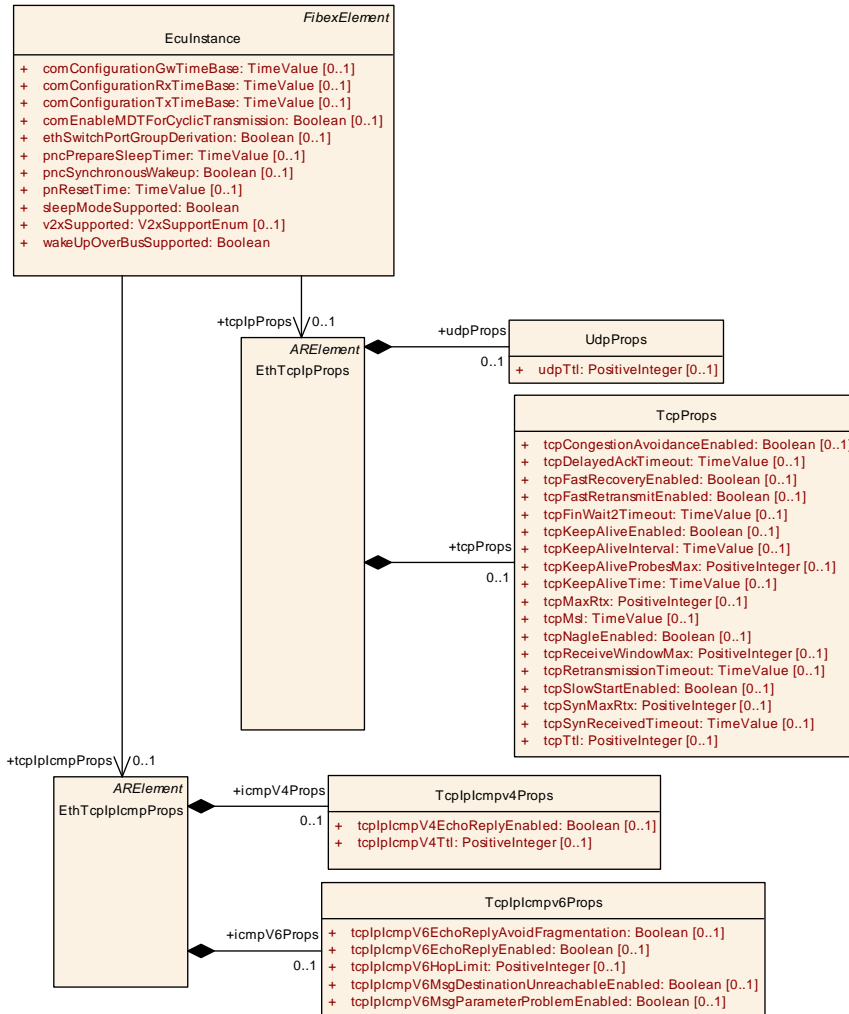
Figure 3.18: Ecu specific TCP/UDP and ICMP configuration options
