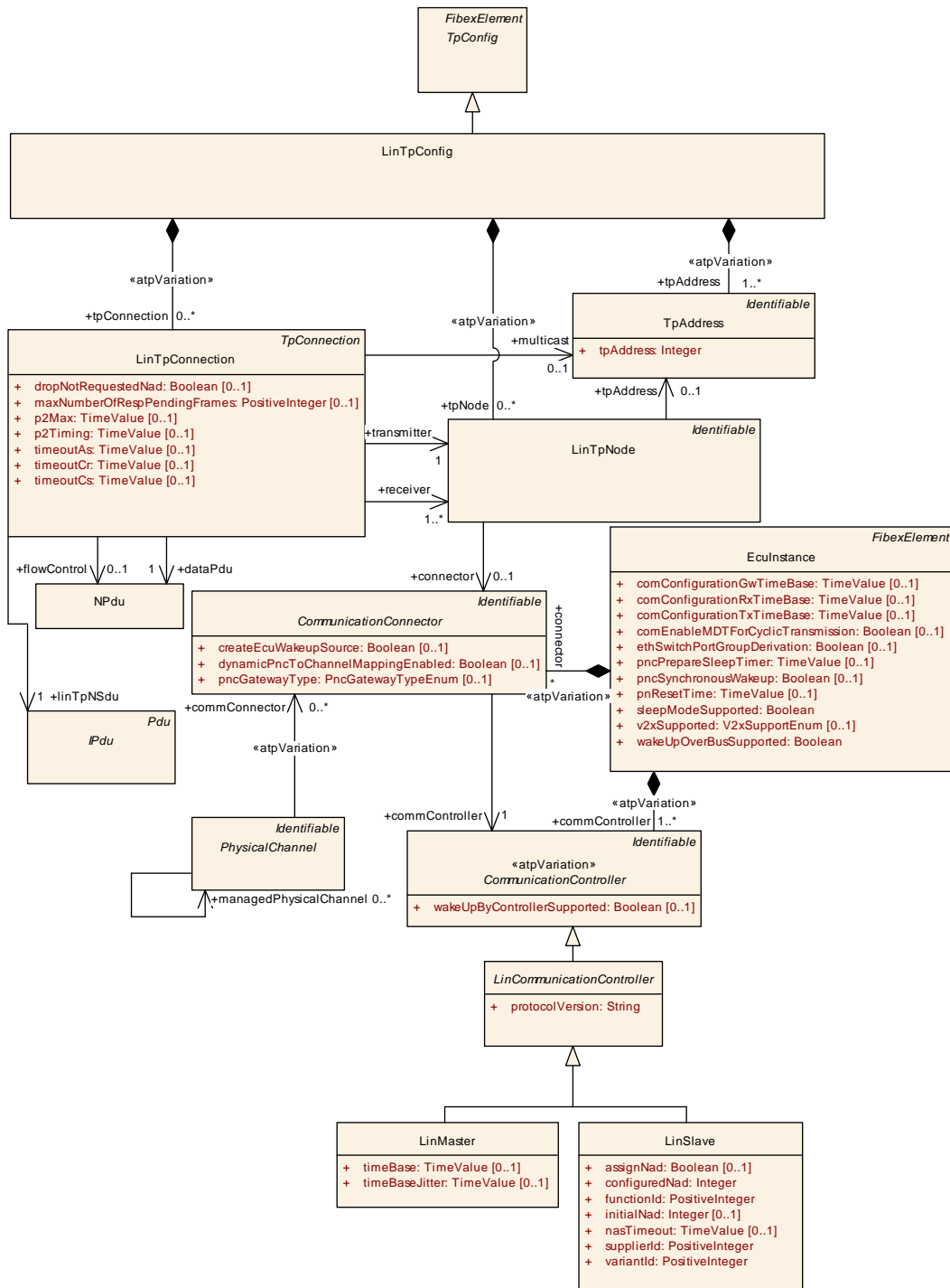
Figure 6.62: LIN Transport Layer Configuration
