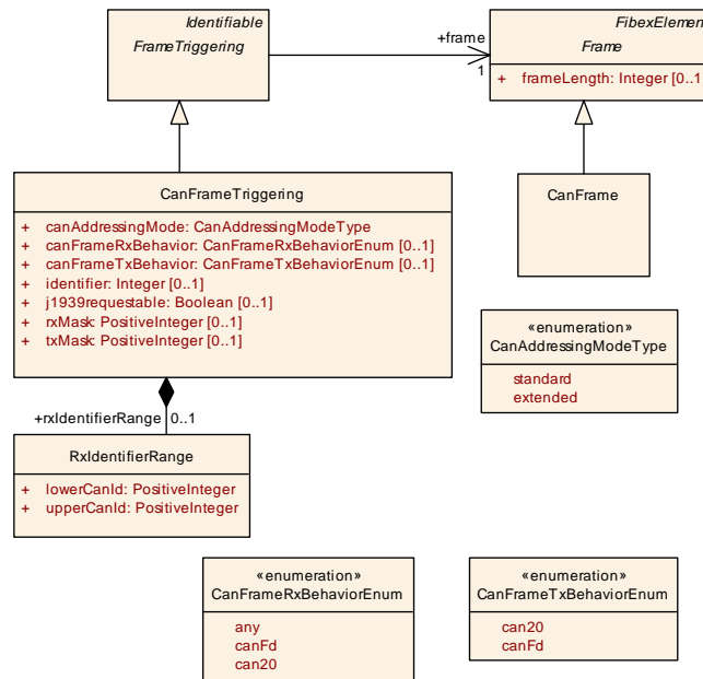
Figure 6.34: CanFrameTriggering (Fibex4Can:CanCommunication)
