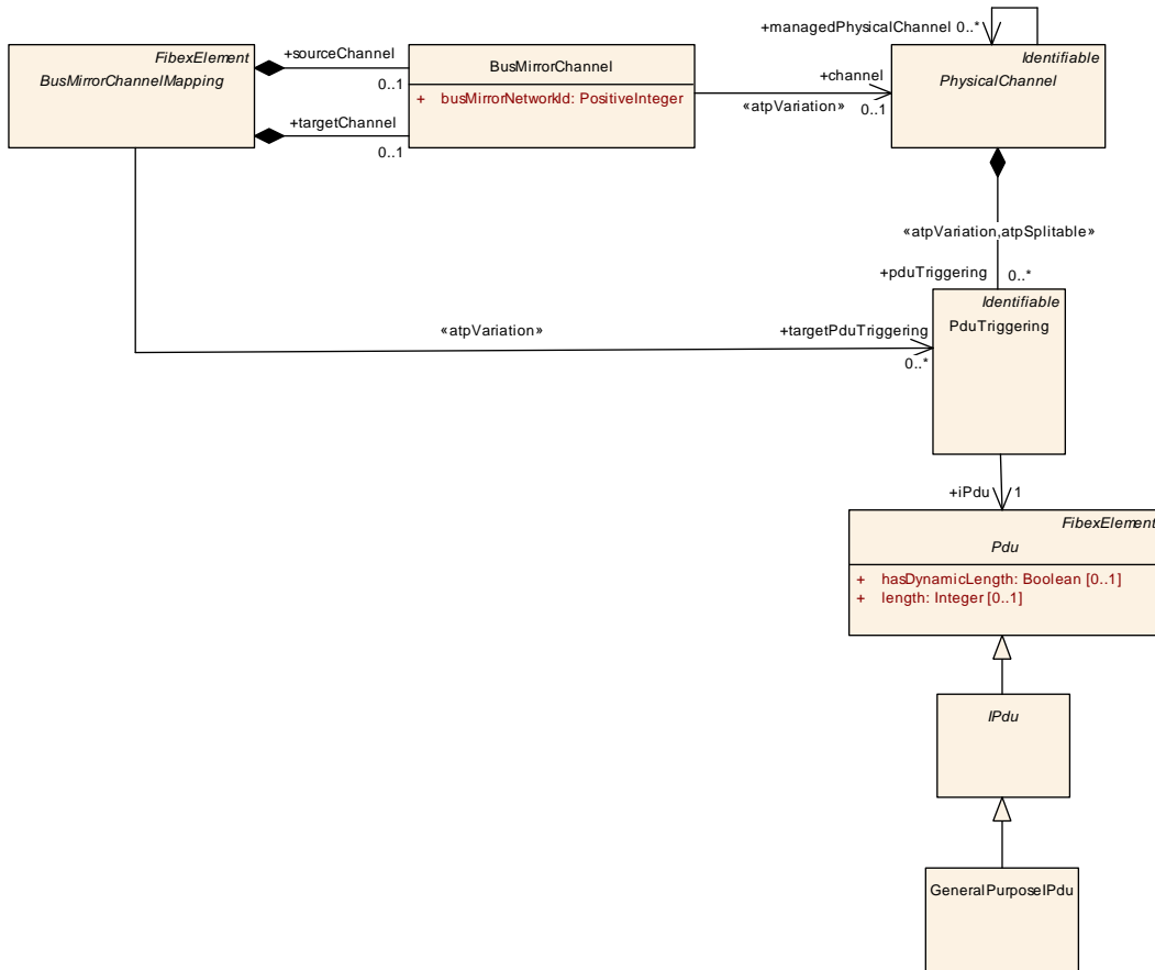
Figure 6.77: Bus mirroring
