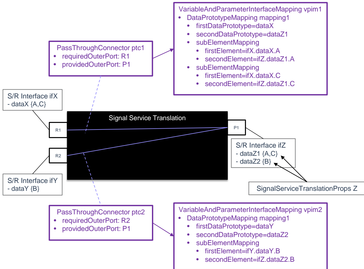
Figure 6.101: Mapping description using PassThroughSwConnectors and PortInterfaceMappings
