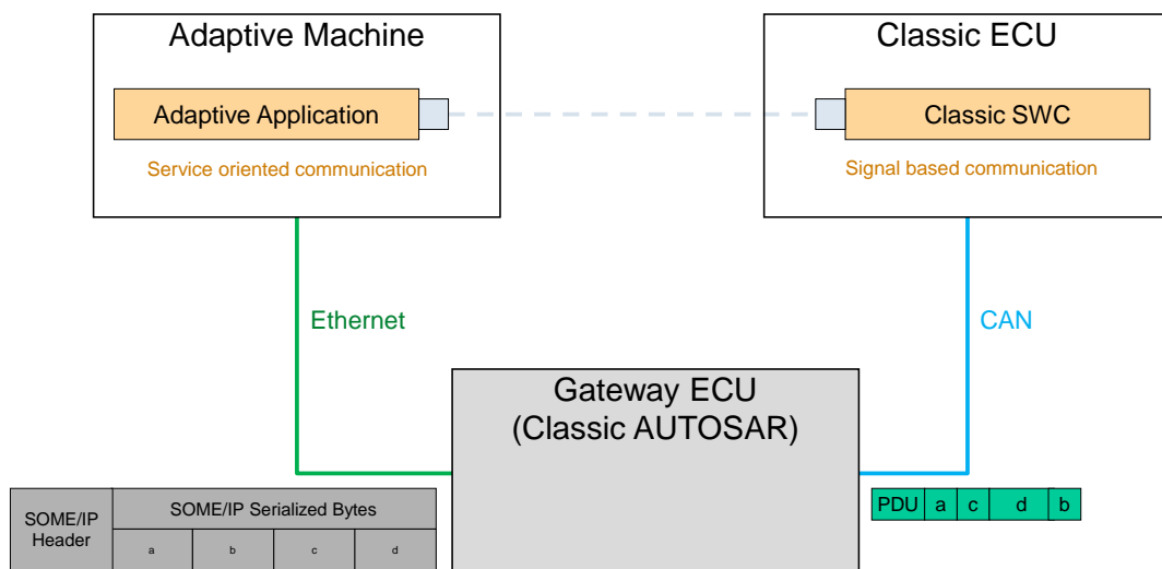
Figure 6.97: Signal Service Translation in Classic platform gateway ECU
