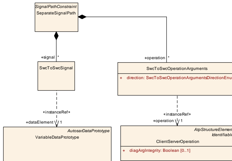
Figure 5.22: Description of signals that shall not take the same way in the topology (SeparateSignalPath)
