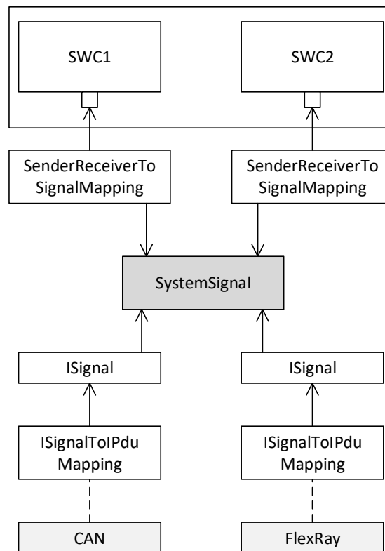
Figure 5.8: Example for a SystemSignal and a DataMapping
