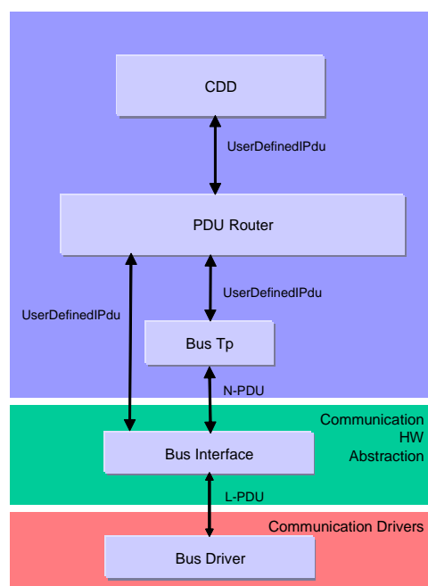
Figure 6.95: CDD over PduR
