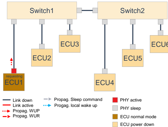
Figure 3.20: While the link is down on the connected dataline, the PHY of ECU1 transmit a wake-up on the network
