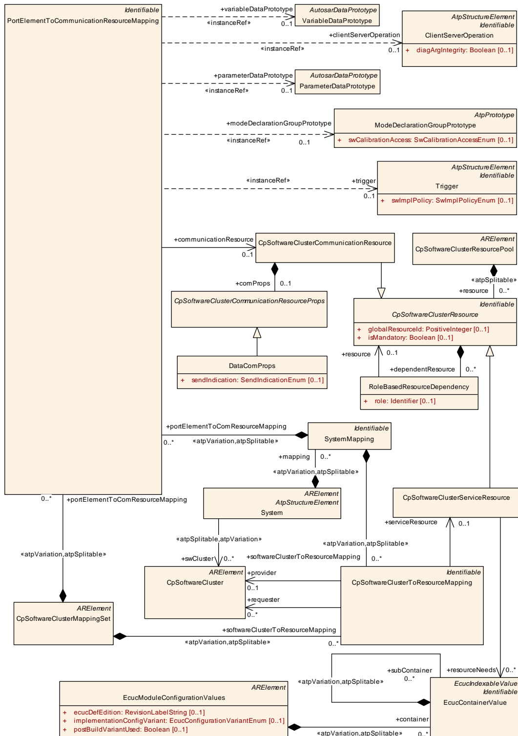
Figure 11.6: Software Cluster Resources
