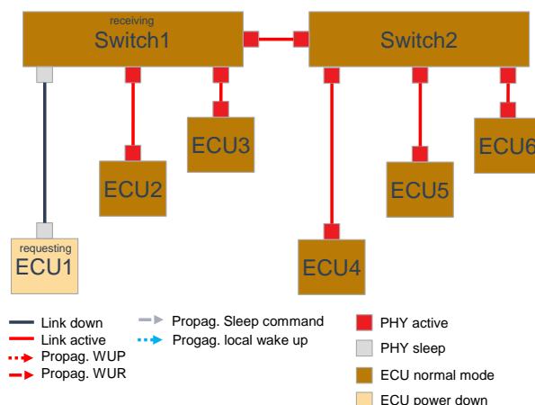
Figure 3.26: ECU1 (requesting ECU) is already in power down mode, while Switch1 is waiting until couplingPortSwitchoffDelay has expired. If couplingPortSwitchoffDelay has expired, Switch1 will detect that the Ethernet hardware is already in sleep state and therefore will NOT trigger a Sleep.request
