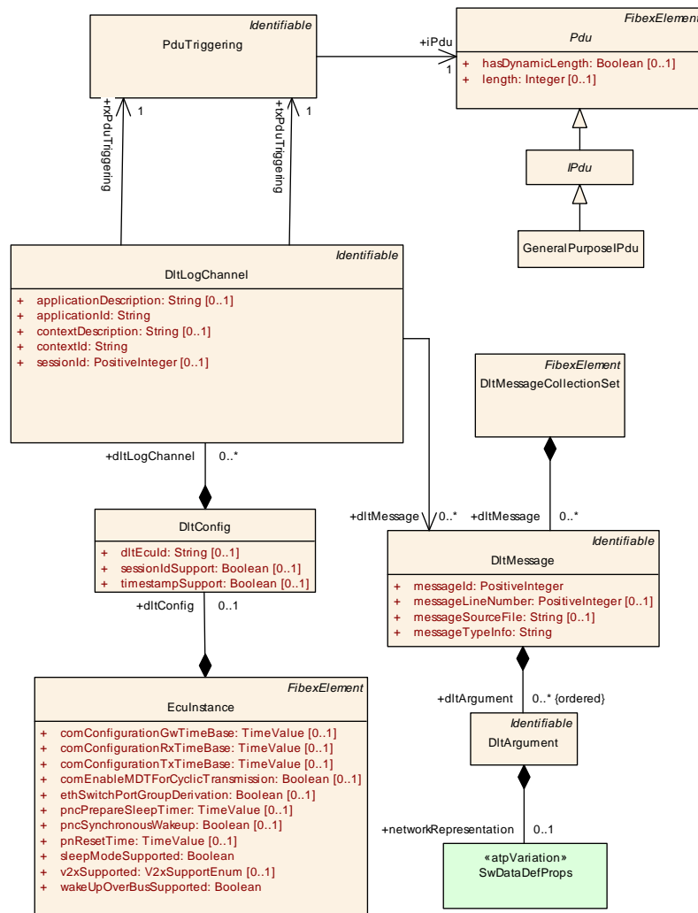
Figure 6.94: Dlt configuration of DltLogChannels and DltMessages
