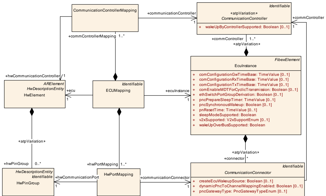
Figure 3.29: Mapping of topology description elements in the System Template onto hardware elements defined in the ECU Resource Template (ECUResourceMapping)
