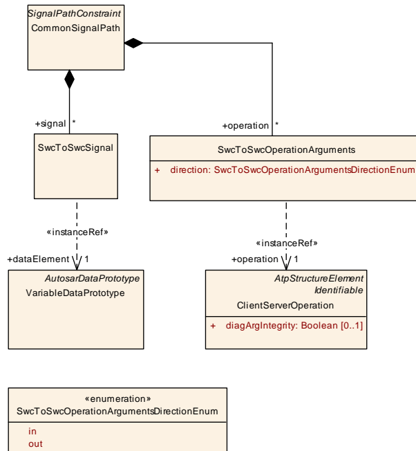
Figure 5.19: Description of signals that shall take the same way in the topology (CommonSignalPath)
