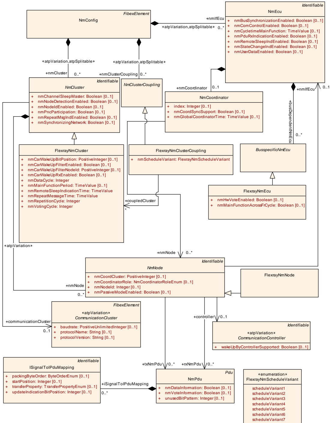
Figure 6.71: FlexRay Network Management Configuration (TransportProtocols: Nm-FlexRayConfiguration)
