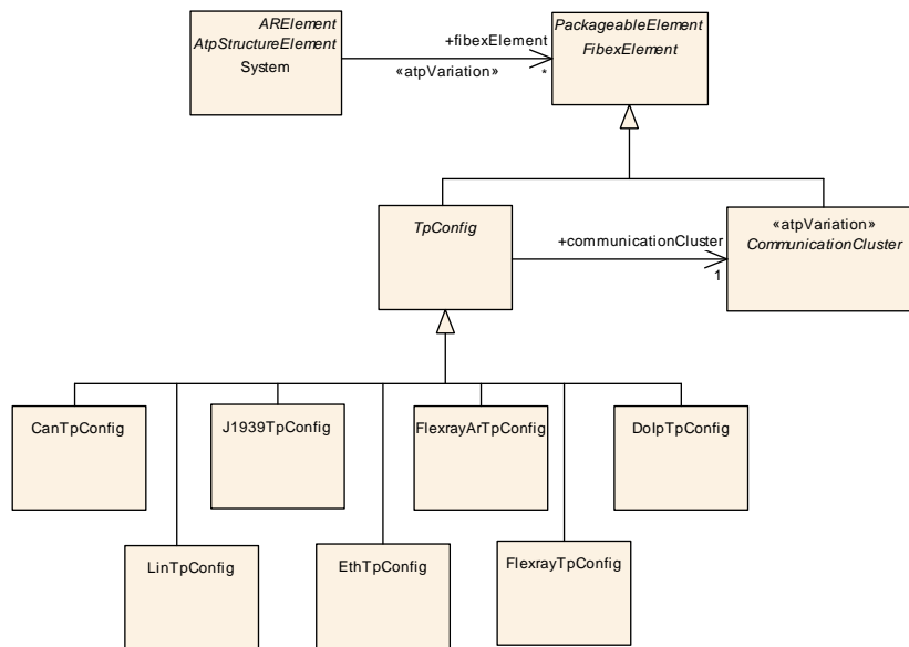
Figure 6.57: Transport Layer Overview
