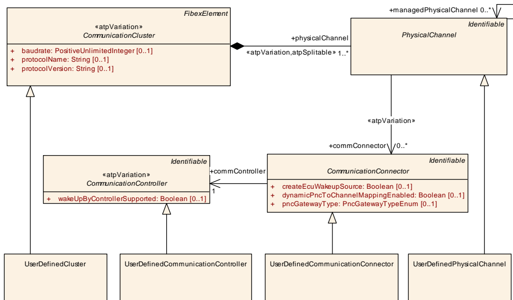
Figure 3.28: User defined topology elements
