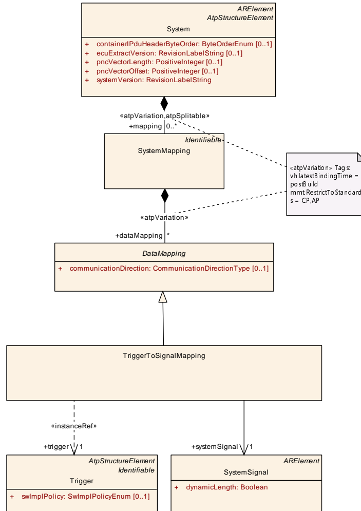
Figure 5.16: Structure of a TriggerToSignalMapping
