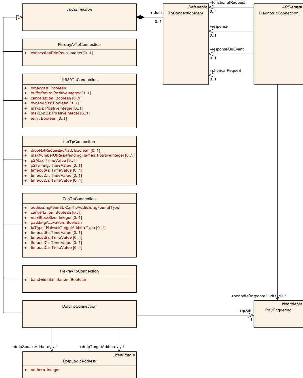
Figure 6.68: Modeling of DiagnosticConnection
