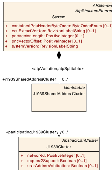
Figure 6.76: J1939SharedAddressCluster
