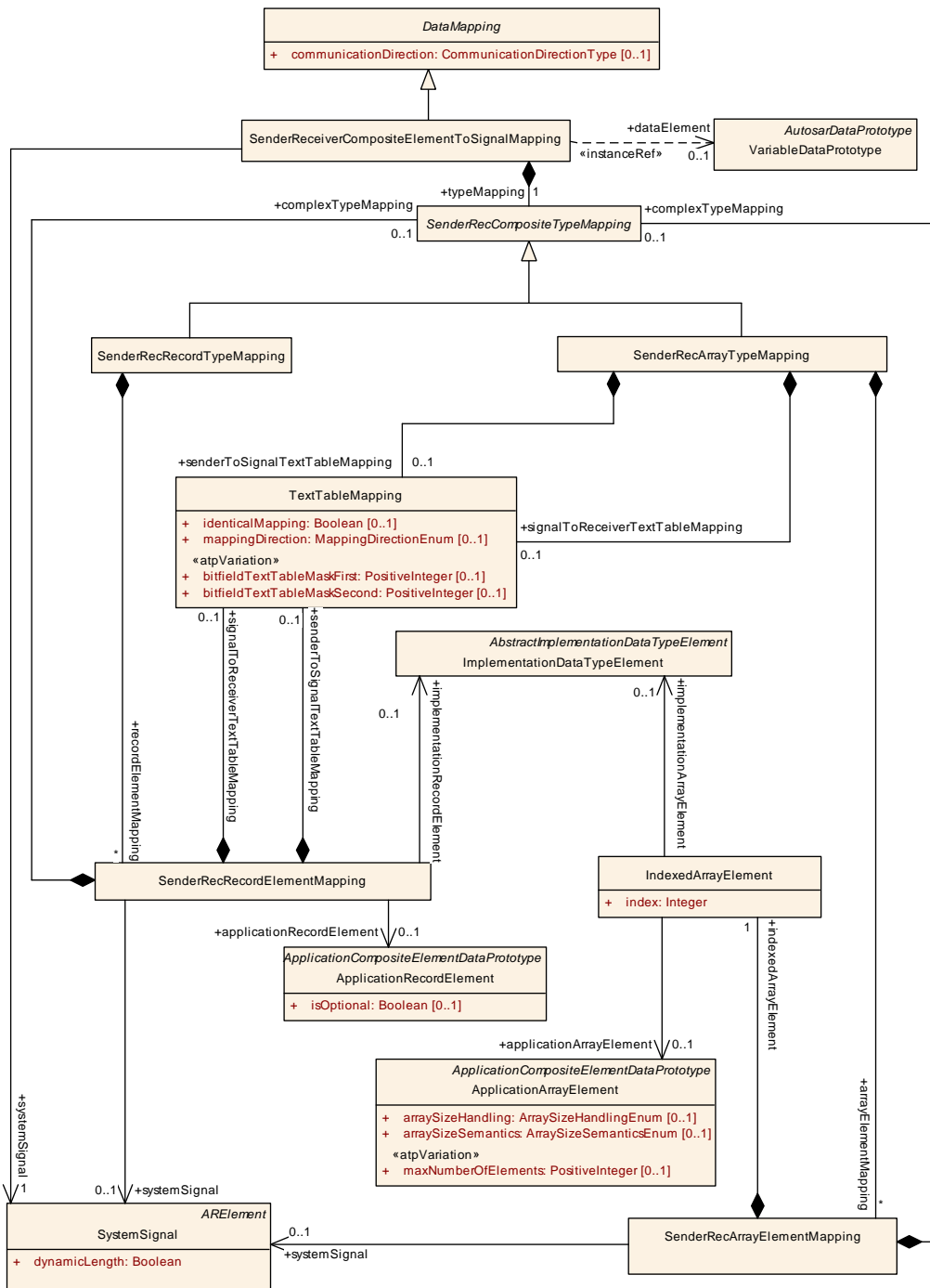
Figure 5.15: Mapping of a Variable Data Prototype which is aggregated within a composite data type on a System Signal
