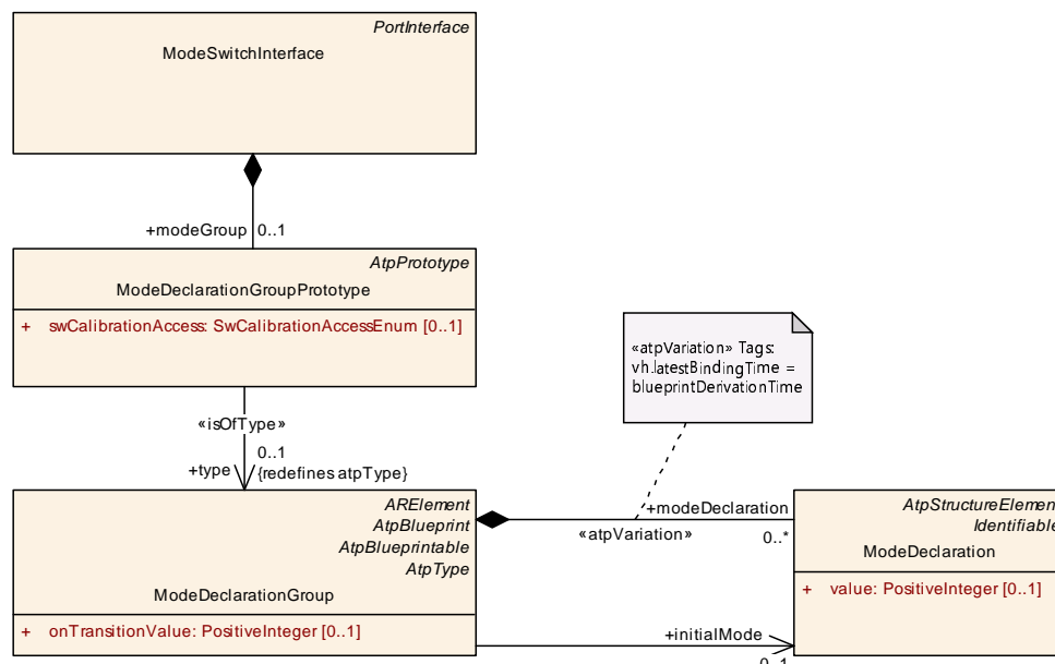
Figure 2.3: mode switch interface
