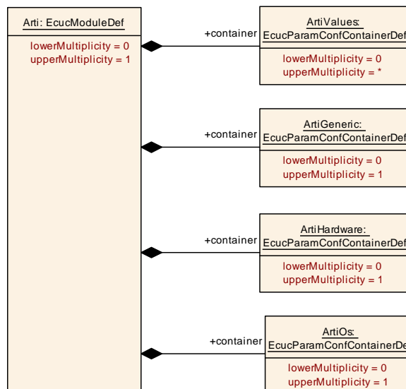
Figure 3.3: Arti Ecuc Module Definition Class Diagram
