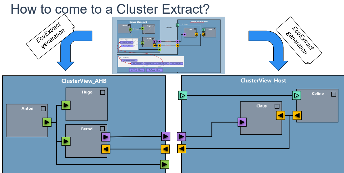
Figure 5.2: Overview of the Software Cluster Extract
