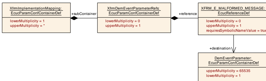
Figure 10.3: AR_EcucDef_XfrmDemEventParameterRefs
