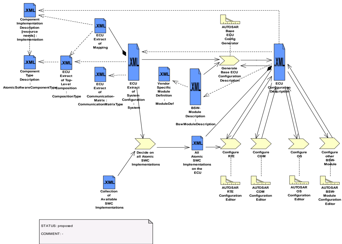
Figure 8 distinguishes only the configuration activities Configure RTE, Configure COM, Configure OS, and Configure other BSW Module, all supported by an appropriate configuration editor 9 .
