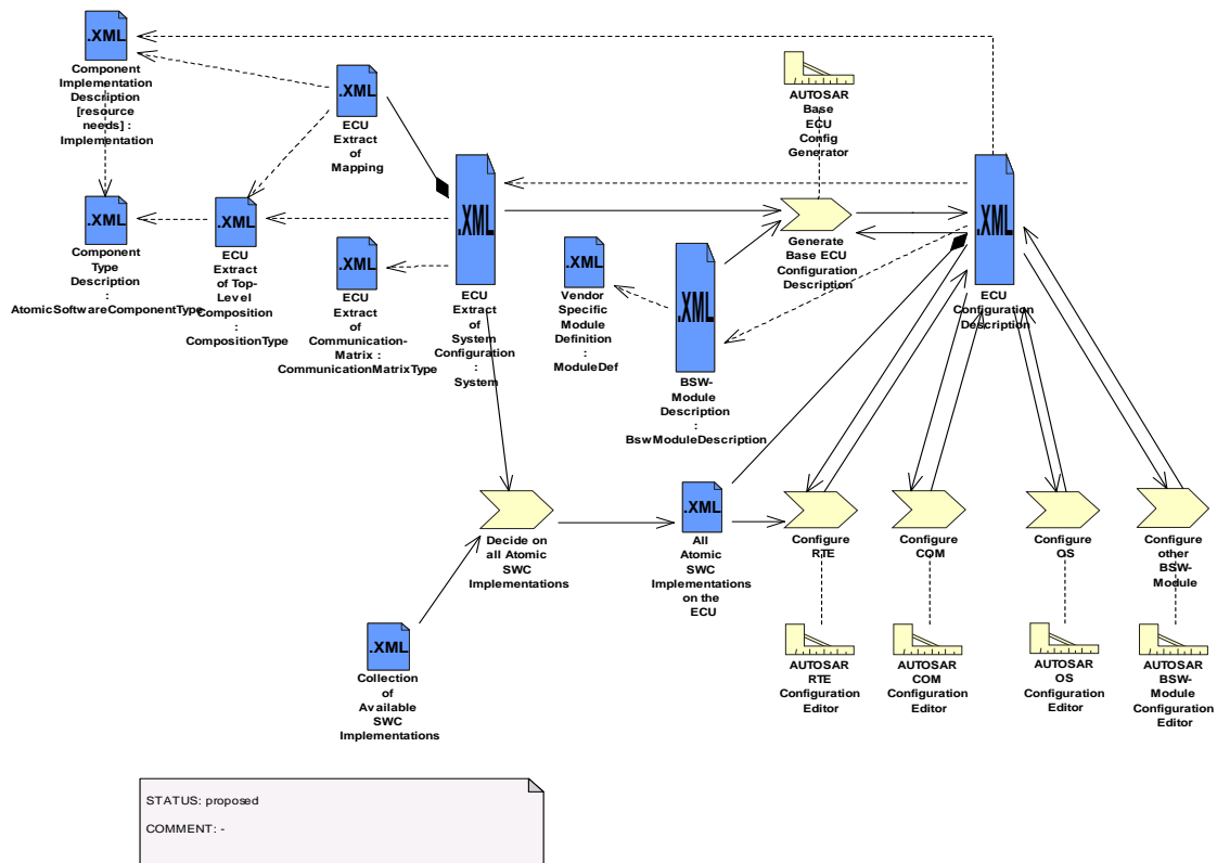
Figure 8 shows the details of the ECU configuration. In regard to the time flow of the ECU configuration, this starts with the activity Generate Base ECU Configuration Description which is supported by the tool AUTOSAR Base ECU Config Generator 8 . This activity takes the input ECU Extract of System Configuration, the BSW Module Description and if existing a previously generated ECU Configuration Description.
