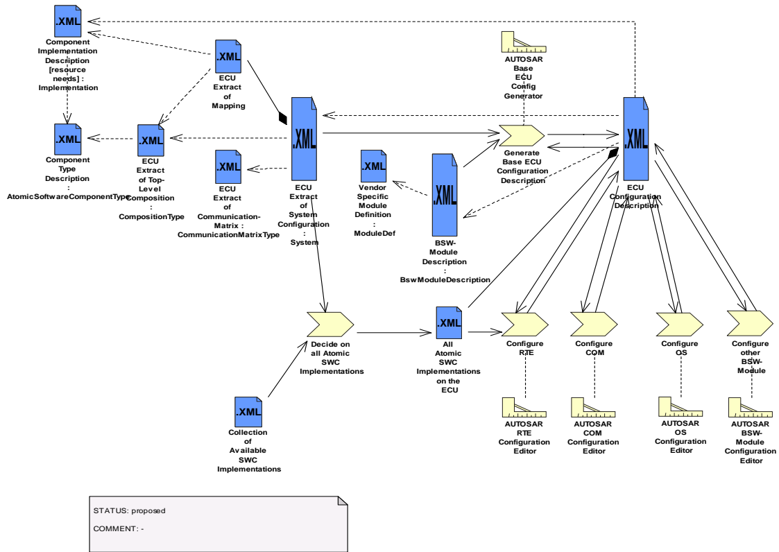
Figure 8 depicts the work products the ECU Extract of System Configuration has to access (either as contained part or via reference) for generating the base configuration. These are ECU specific extracts of the top-level composition, the mapping and the communication matrix.
