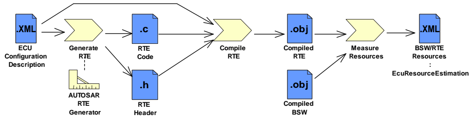
Figure 10: Per-ECU RTE generation
