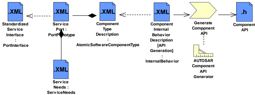
Figure 14: Per service part of AUTOSAR methodology
