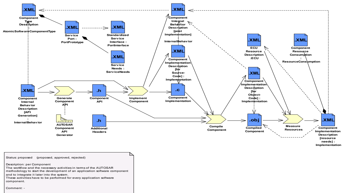
Figure 13: Per component part of the AUTOSAR methodology
