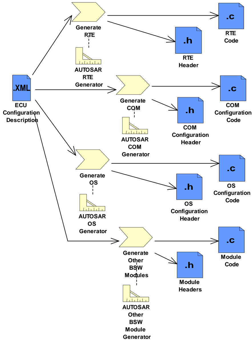
Figure 9: Per-ECU Basic Software generation
