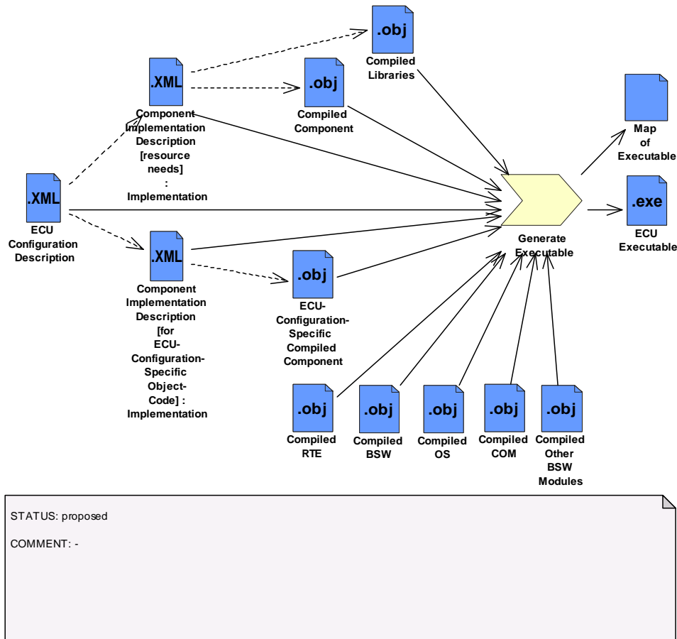
Figure 11: Generation of executable code for ECU
