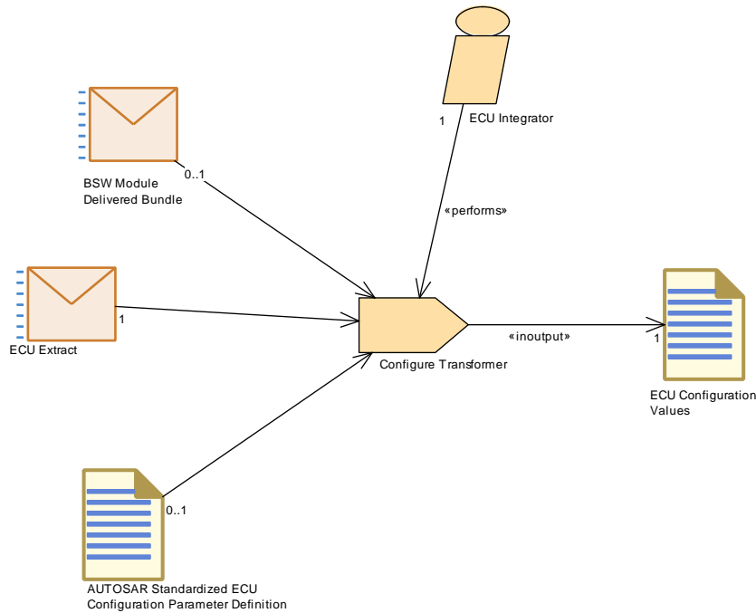
Figure 3.139: Configure Transformer
