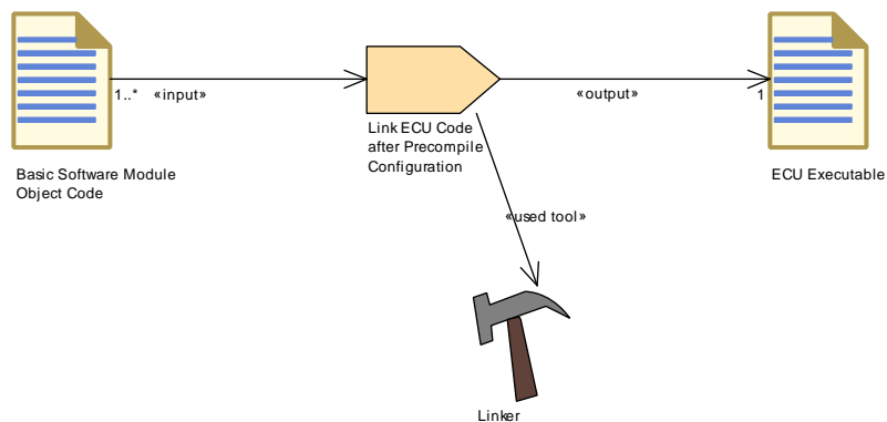
Figure 3.163: Link ECU after Precompile Configuration
