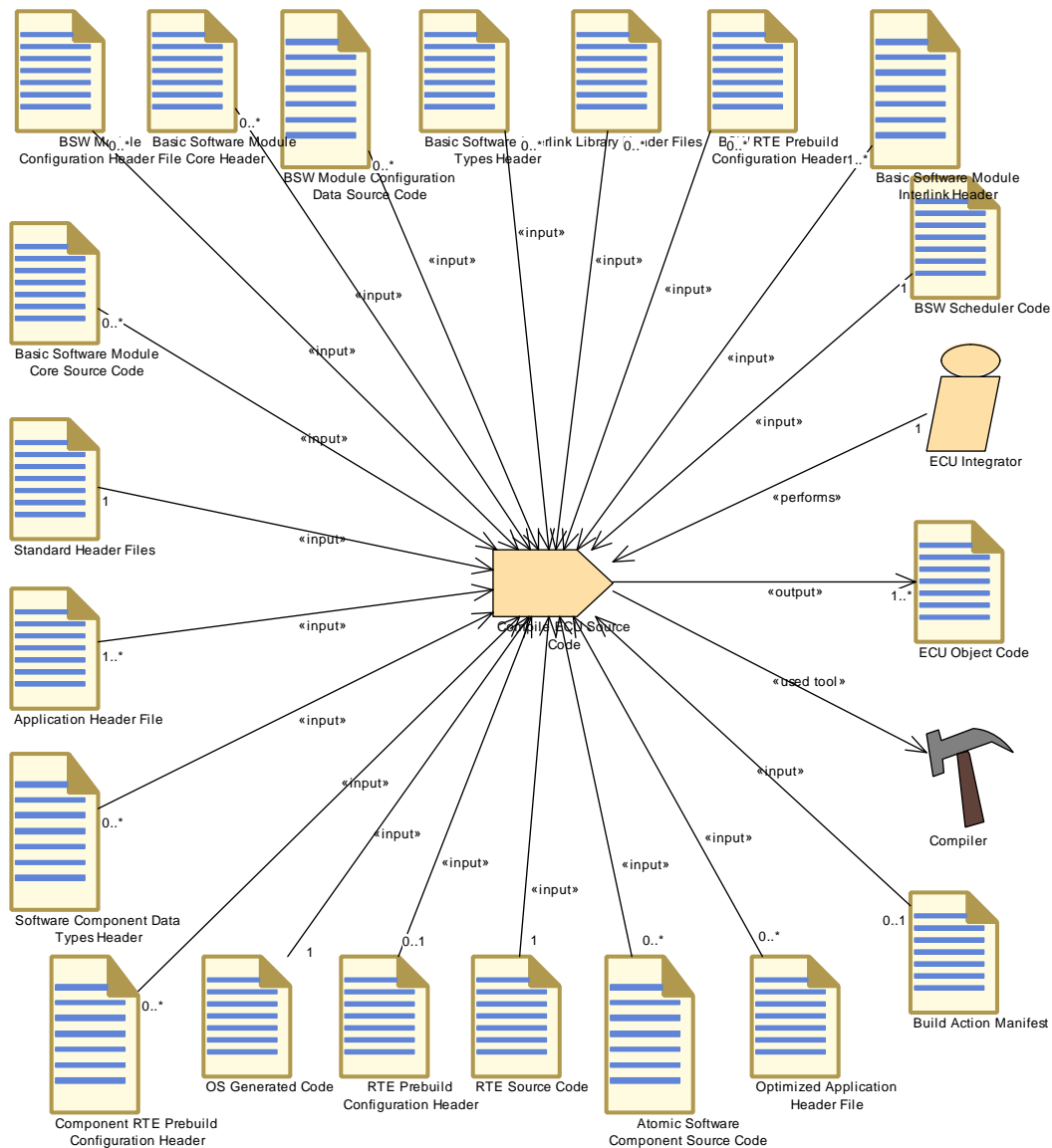
Figure 3.147: Compile ECU Source Code
