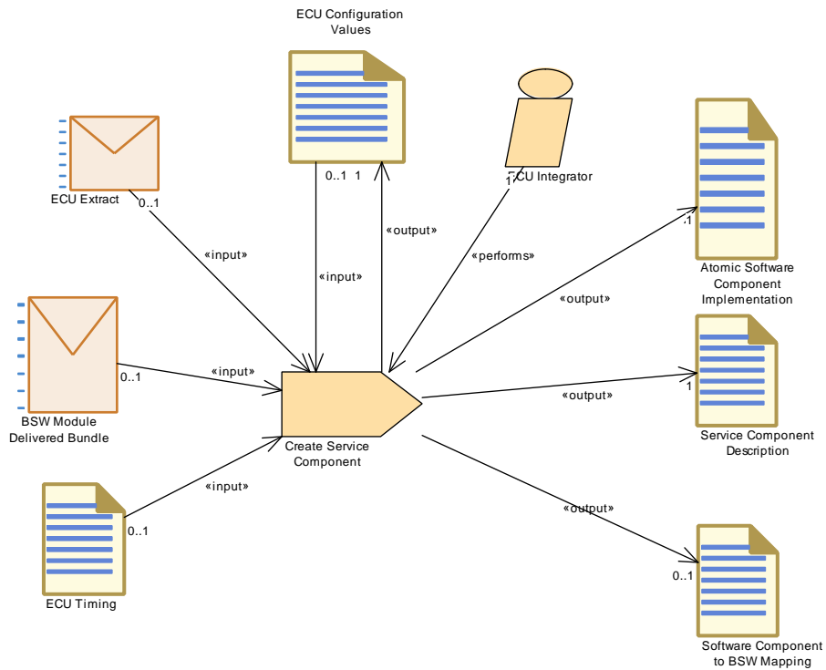
Figure 3.134: Create Service Component
