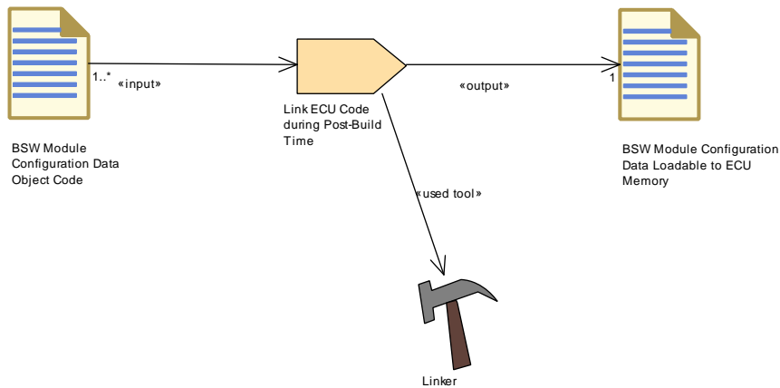
Figure 3.165: Link ECU Code During Post-build Time
