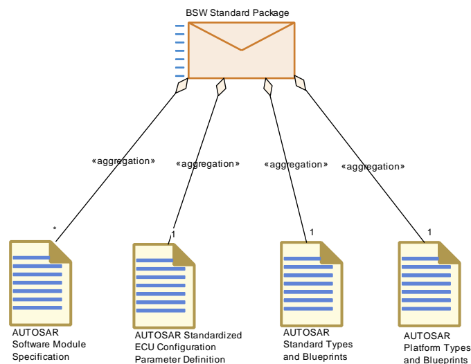
Figure 3.118: BSW Standard Package
