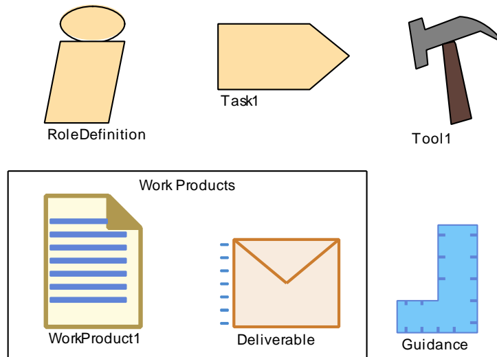
Figure 1.1: Symbols of AUTOSAR Methodology Library Element
