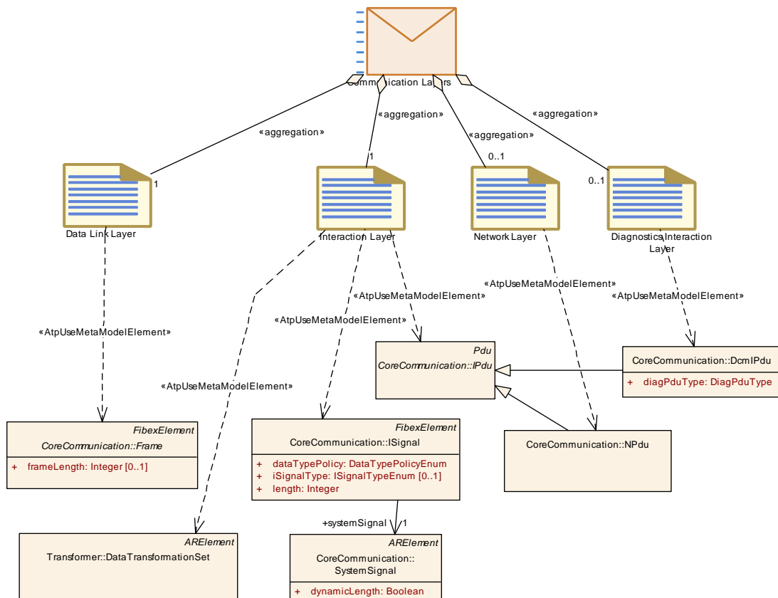
Figure 3.80: Communication Layers
