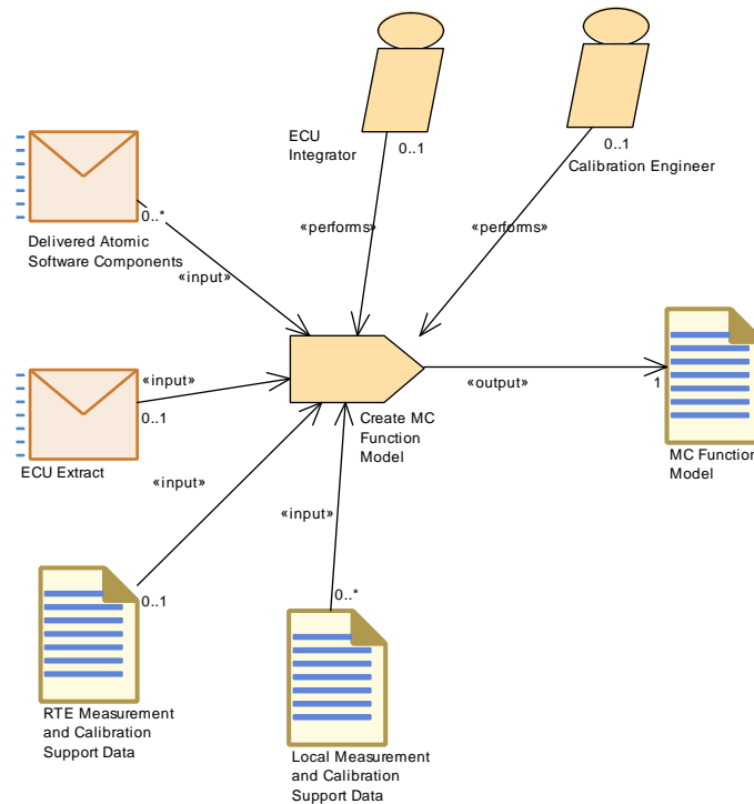
Figure 3.142: Create MC Function Model
