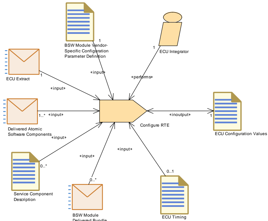
Figure 3.129: Configure RTE
