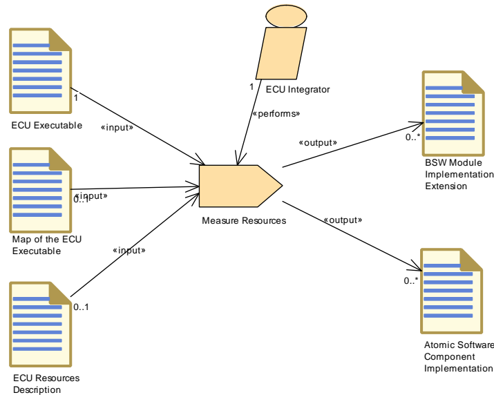
Figure 3.151: Measure Resources
