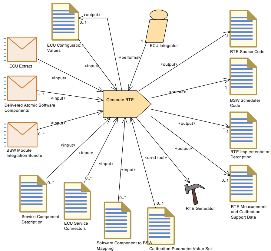
Figure 3.143: Generate RTE
