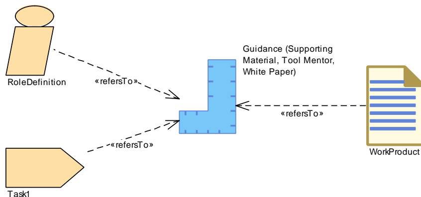
Figure 1.6: Guidance Overview
