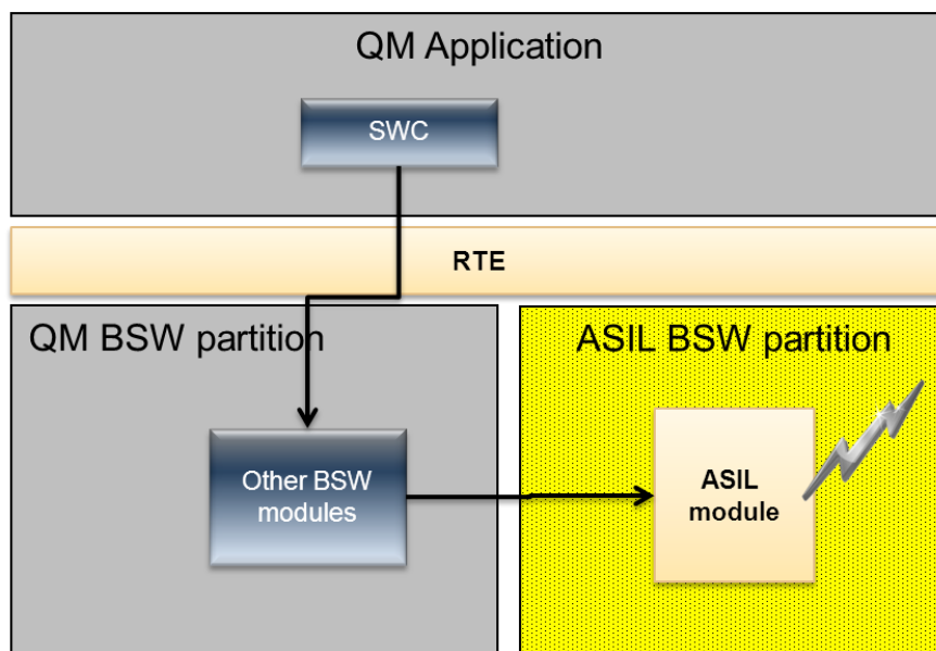
Figure 33: Timing fault
