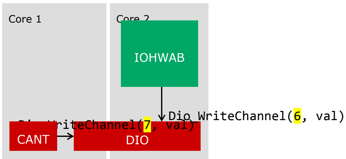
Figure 18 - Example 2 - DIO – Accessed by CanTrcv and IoHWAb on Different Cores
