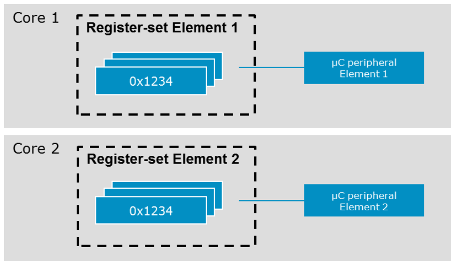
Figure 10 - Independent Register-Set HW Level Separation
