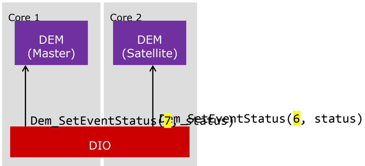
Figure 19 - Example 3 - DIO - Accessed by Dem Master and Satellite
