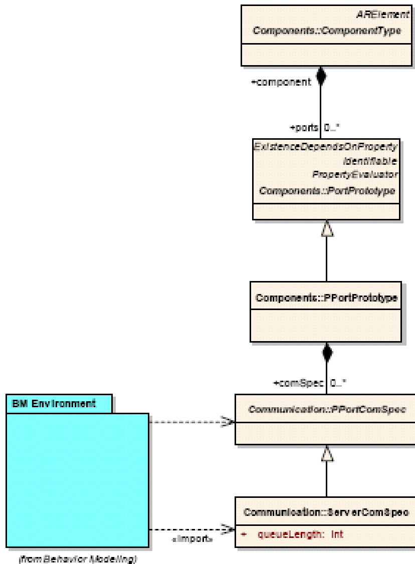
Figure 17: ServerComSpec
