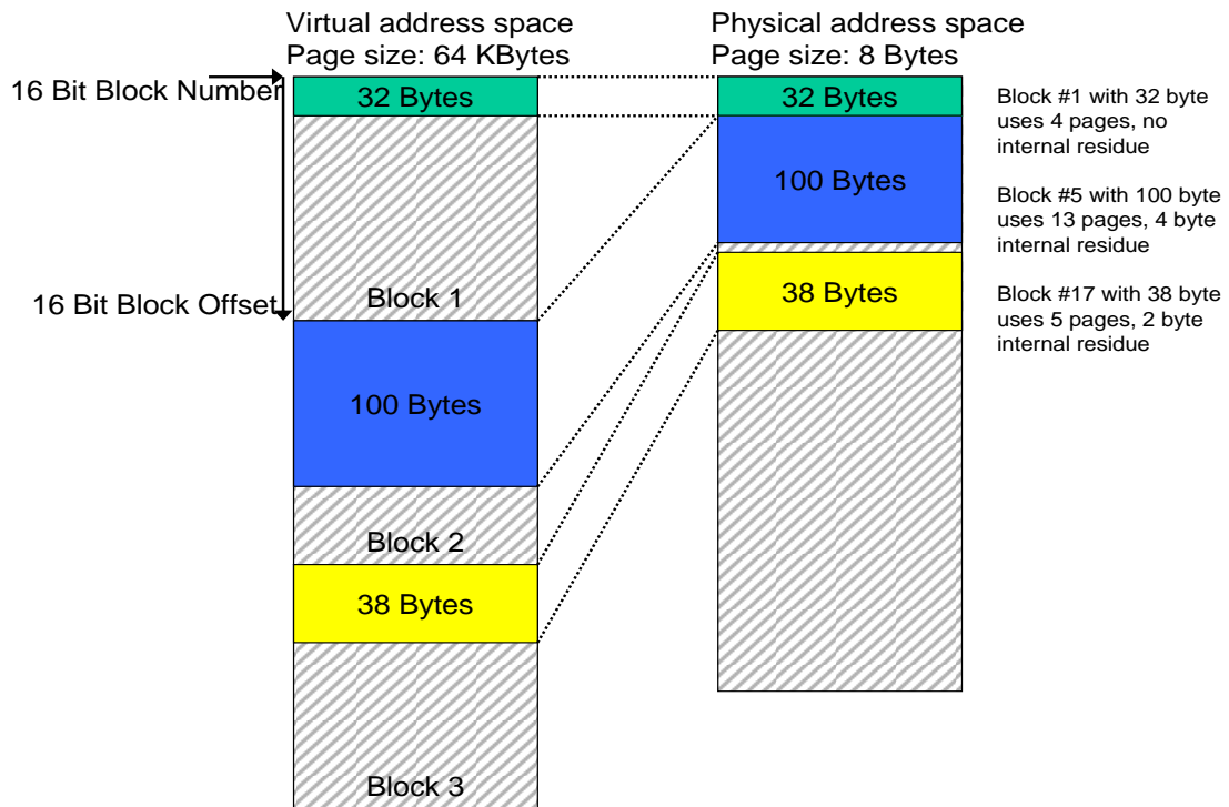
Figure 2: Virtual vs. physical address space
