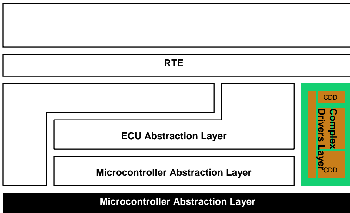
Figure 4.2-1: CDD in Layered Software Architecture
