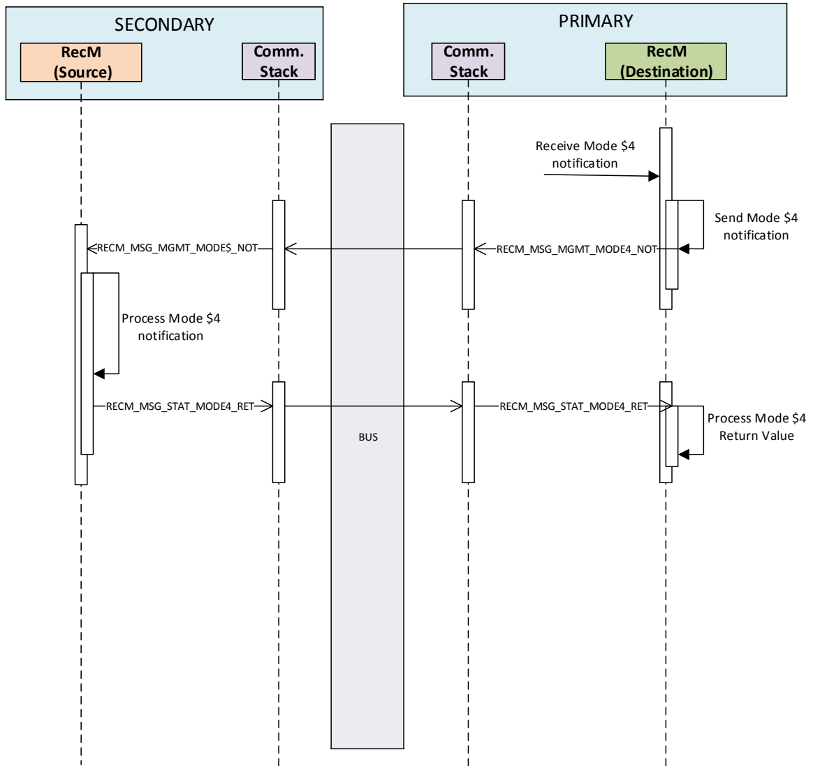
Figure 5.11: Sequence diagram of Process Mode $04 Notification
