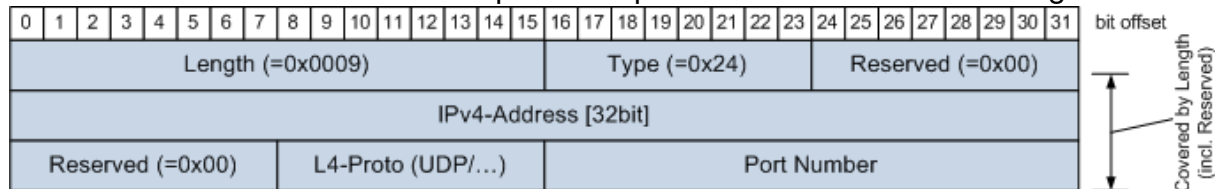
Figure 4.13: SOME/IP-SD IPv4 SD Endpoint Option
