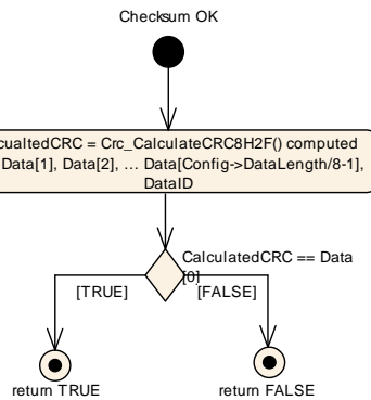
Figure 6.12: Checksum OK
