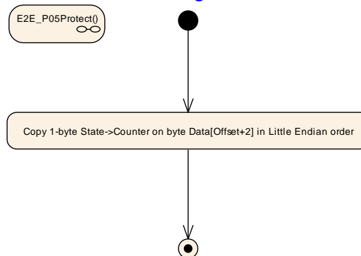
Figure 6.35: E2E Profile 5 Protect step "Write Counter"
