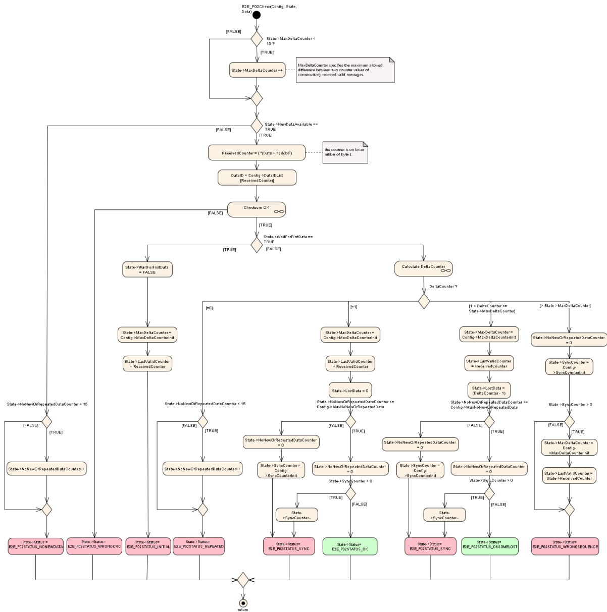
Figure 6.11: E2E_P02Check
