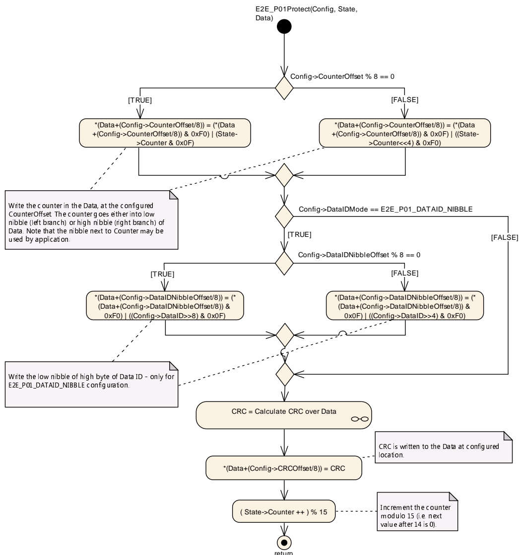
Figure 6.5: E2E_P01Protect()
