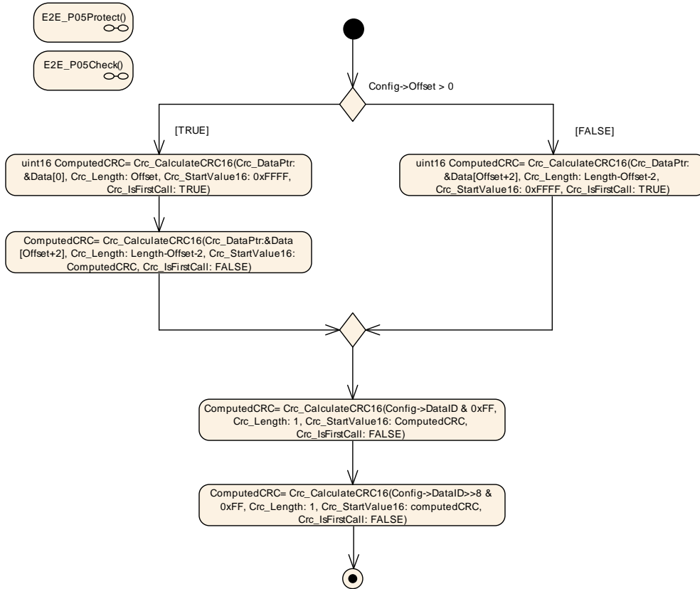
Figure 6.36: E2E Profile 5 Protect and Check step "Compute CRC"
