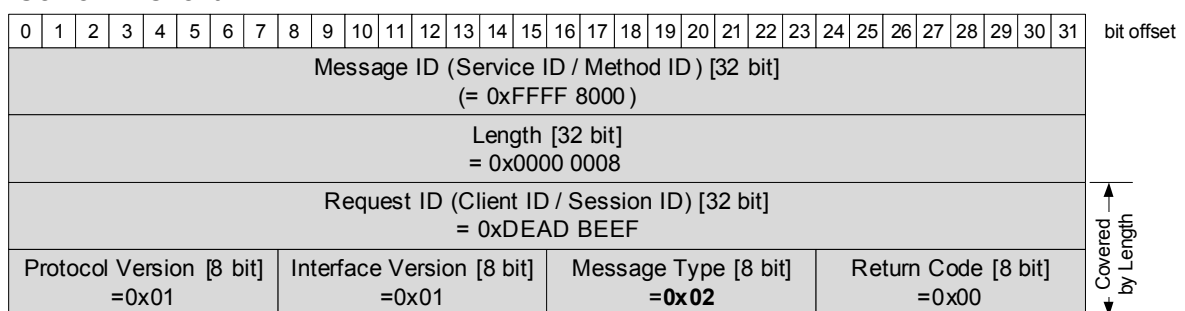
Figure 4.14: SOME/IP Magic Cookie Message for SOME/IP
